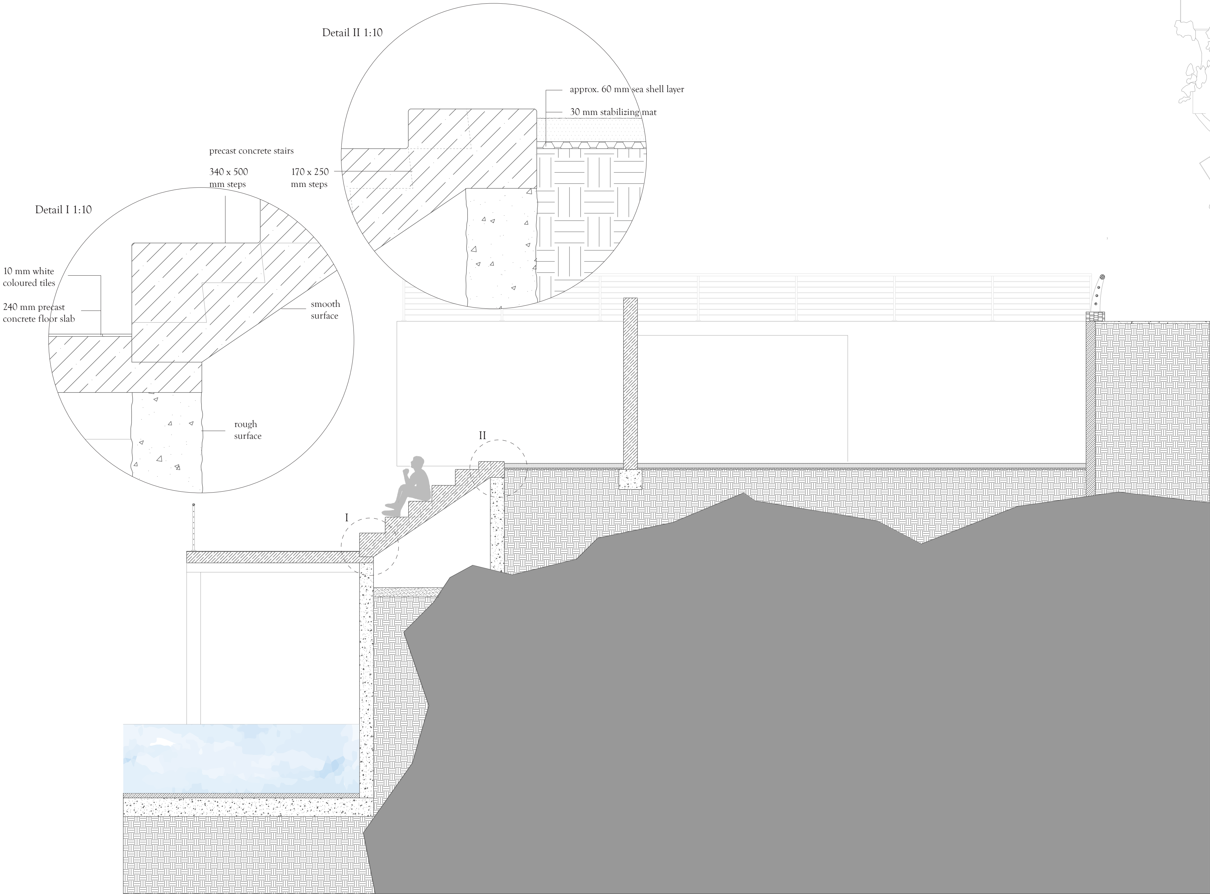
Section A 1:50
