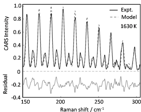
Fig. 3. Single-shot, femtosecond/picosecond resonant CARS spectrum, generated as short pump-probe pulse delay ( \sim 3\text{ps} ) and acquired at \sim 450 \text{ }\mu\text{m} from the flame-front of a premixed methane/air flame ( \Phi=0.95 ). The resonant spectrum, acquired in first detection channel, was back-ground subtracted and referenced to the non-resonant CARS spectrum acquired simultaneously in the second detection channel. In order to determine the corresponding temperature, the resulting spectrum was compared to a library of synthetic spectra, computed by means of a time-resolved CARS code. The resulting temperature in the measurement location was thus assessed in 1630 K. The performance of the spectral fitting can be evaluated by the residuals of the theoretical and experimental spectra, which are presented in the figure, with an offset of -0.2 for clarity purposes.
