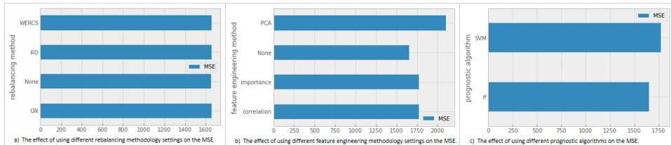
Figure 4.8: A comparison of applying the different prognostic settings on dataset FD001.
