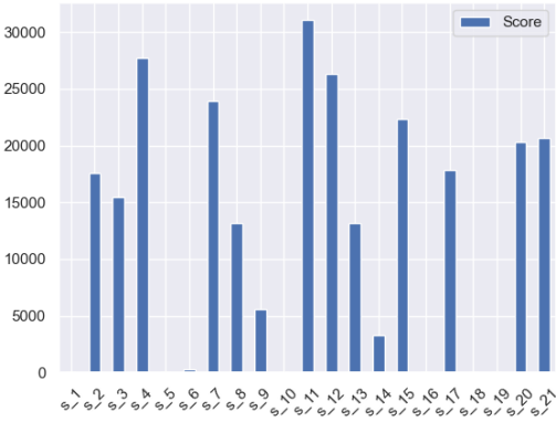
Figure 4.6: The features selected by the PCA and their relevance scores (the higher the more relevant).
