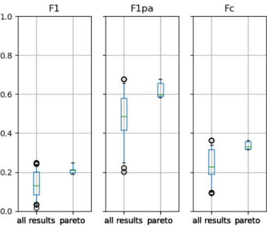
Figure 3.6: Scores of all individuals and Pareto front individuals for SMAP dataset.
