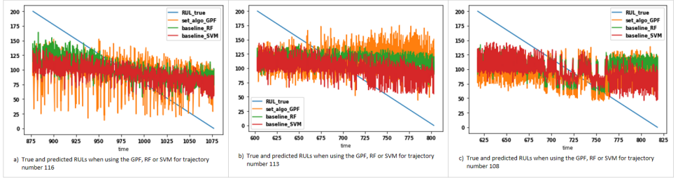
Figure 4.18: True and predicted values for three different trajectories of the SCU test set when using the GPF, RF and SVM (cut 200 FC before failure).
