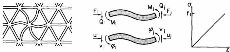
Figure 3.14: (left) Regular triangular lattice of beams, (middle) external forces and deformations on a single beam element, and (right) stress-strain relation for an element [17]
