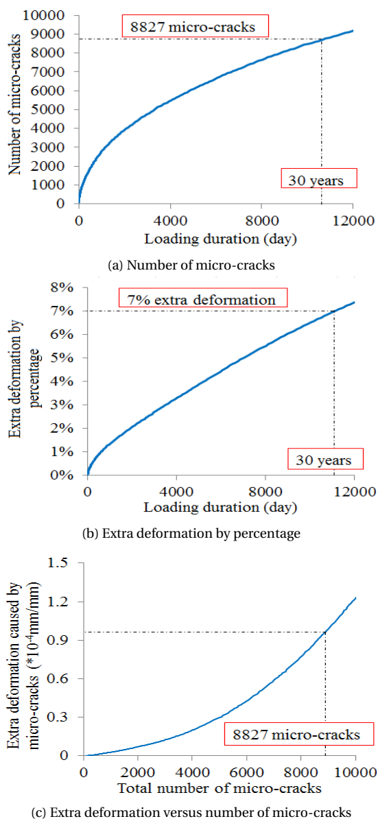
Figure 3.31: (a) Total number of cracks during the creep process; (b) Percentage of additional deformation caused by micro-cracking [extra deformation by percentage = (deformation with micro-cracking - deformation without micro-cracking) / deformation without micro-cracking]; (c) The extra deformation caused by micro-cracking versus total number of micro-cracks
