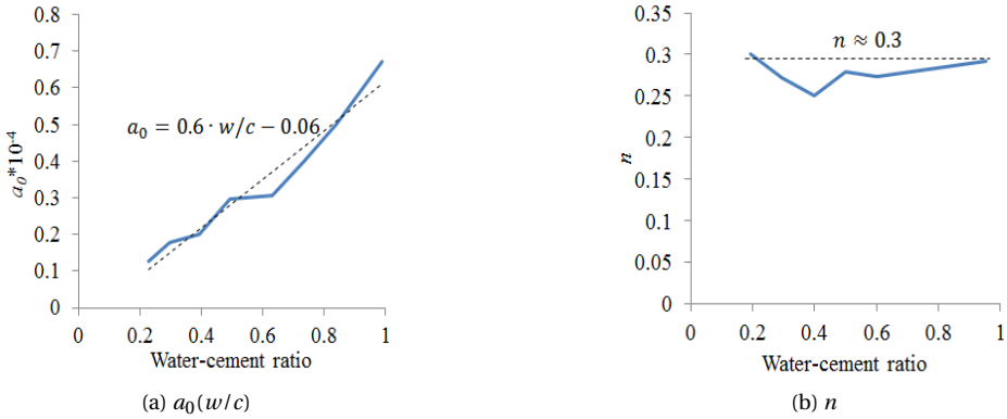
Figure 4.9: Parameter a_0 , n as a function of water-cement ratio (age at loading = 35 days; stress-strength ratio = 0.3; stress is constant) [20, 21]
