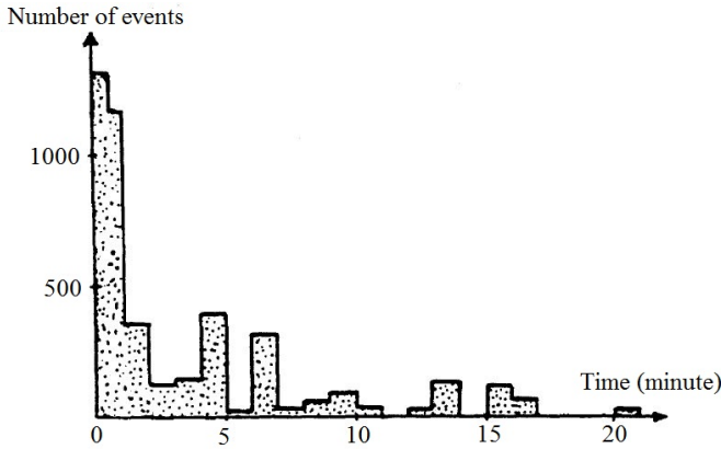
Figure 2.6: Acoustic emission obtained during a basic creep test (note: first 20 minutes) [8]
