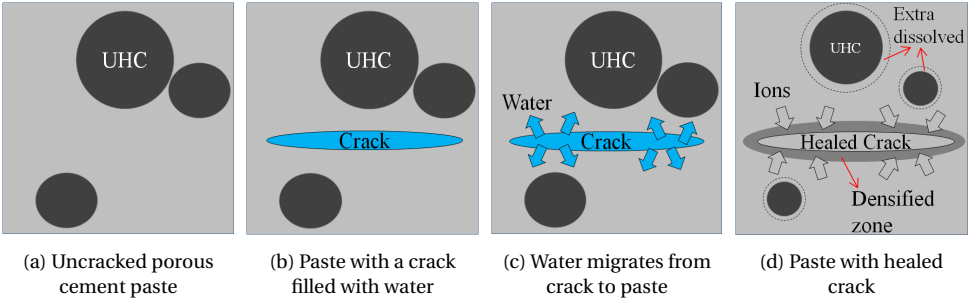
Figure 3.4: Schematic diagram illustrating the self-healing mechanism for the extra strength increase in concrete under sustained load: (a) Un-cracked porous cement paste; (b) Cracked cement paste (water does into the crack due to capillary suction); (c) Migration of water from the crack into the paste; (d) Dissolution of unhydrated cement grains (uhc), diffusion of the ions to the crack and the pore solution in the paste adjacent to the crack, precipitation of ions in the crack and the paste adjacent to the crack.
