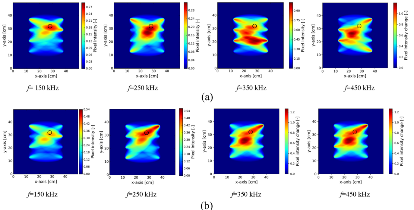
Fig. 12. Image reconstruction at load cycle LC4 for different excitation frequencies, a) DI Pearson , and b) DI Energy .
