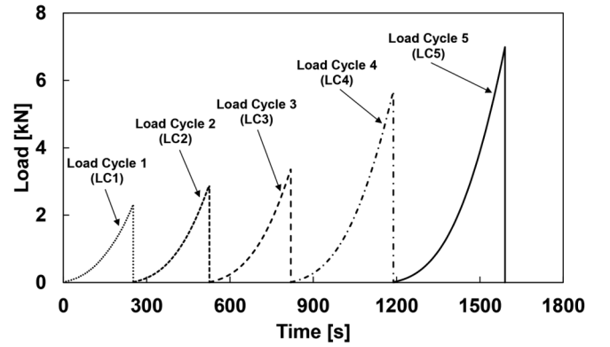
Fig. 3. The sequential increasing indentation load.
