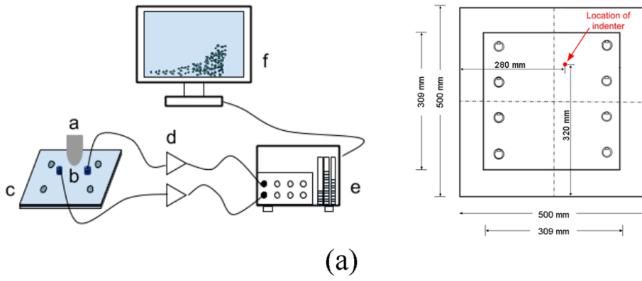
Fig. 4. a) The schematic of impact location and configuration of sequential indentation tests (test apparatus description: (a) indenter, (b) AE sensors, (c) composite panel, (d) preamplifiers with a gain of 34 dB, (e) Vallen AMSY-6 acoustic signal processor, and (f) laptop with Vallen Acquisition and Vallen Visual TM software), and b) the experimental test apparatus for sequential indentation tests.
