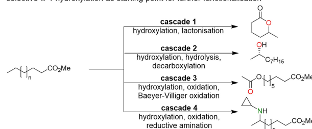
Scheme 1. Established fatty acid valorisation approaches utilise existing functionalities such as the carboxylate group or pre-existing C=C-double bonds. In this contribution we add functionality via selective, peroxygenase-catalysed hydroxylation enabling further transformations.
