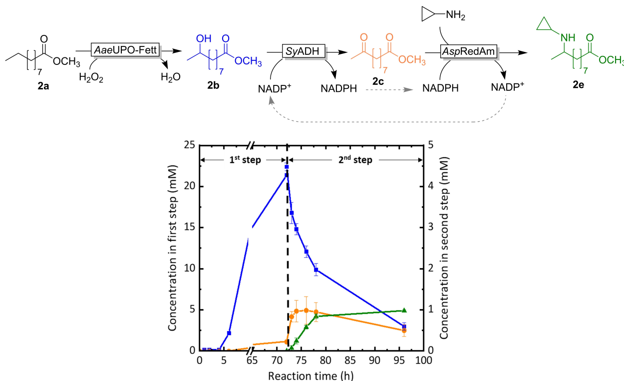
Figure 6. Proposed enzymatic cascade reaction to convert methyl decanoate into methyl 9-cyclopropylaminodecanoate (▲), with the intermediate methyl 9-hydroxydecanoate (■) and methyl 9-oxo-decanoate (●) catalysed by AaeUPO–Fett, SyADH and AspRedAm. Reaction conditions: for the first step (0–72 h), [AaeUPO–Fett] = 1 \mu M, methyl decanoate/buffer = 1 : 4 (v/v), 50 mM KPi buffer (pH 7.0), [H 2 O 2 ] = 2 mM \times h –1 , 1000 rpm, 25 °C, 1 mL scale. For the second step (72 h–96 h), [methyl 9-hydroxydecanoate] = 5 mM, [SyADH cells] = 0.5 mg \times mL –1 , [AspRedAm purified enzyme ] = 0.8 mg \times mL –1 , [DMSO] = 2% (v/v), [NADP + ] = 1 mM, [cyclopropylamine] = 40 mM, 100 mM Tris–HCl (pH 9.0), 300 rpm, 25 °C, 1 mL scale. Values represent the average of duplicates (n = 2). Error bars indicate the standard deviation.
