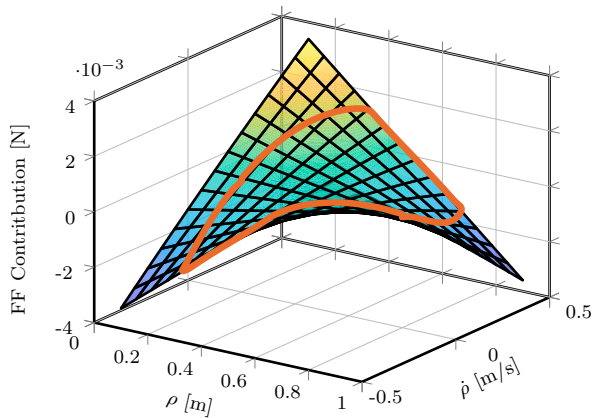
Fig. 6. True dynamic contribution u_{dyn} from (24) and estimated given the data (—) for \ddot{r} = 1 and \dot{r}' = 20 .
