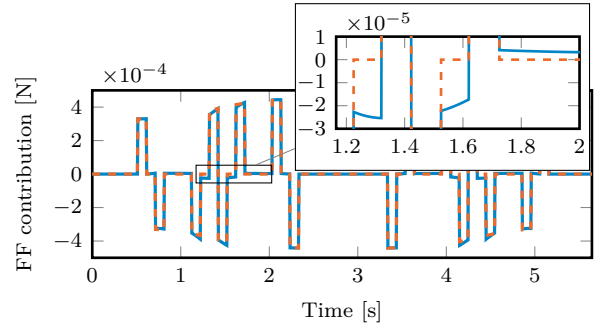
Fig. 5. Feedforward contribution of static LPV \theta_3(\rho) \ddot{r} (---) and developed approach \frac{d^2}{dt^2} (\theta_3(\rho) \ddot{r}) (—). Note that the difference is solely caused by the dynamic scheduling dependency.
