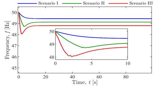
Fig. 4. Scenario I: Frequency response of winter peak operation scenario.
