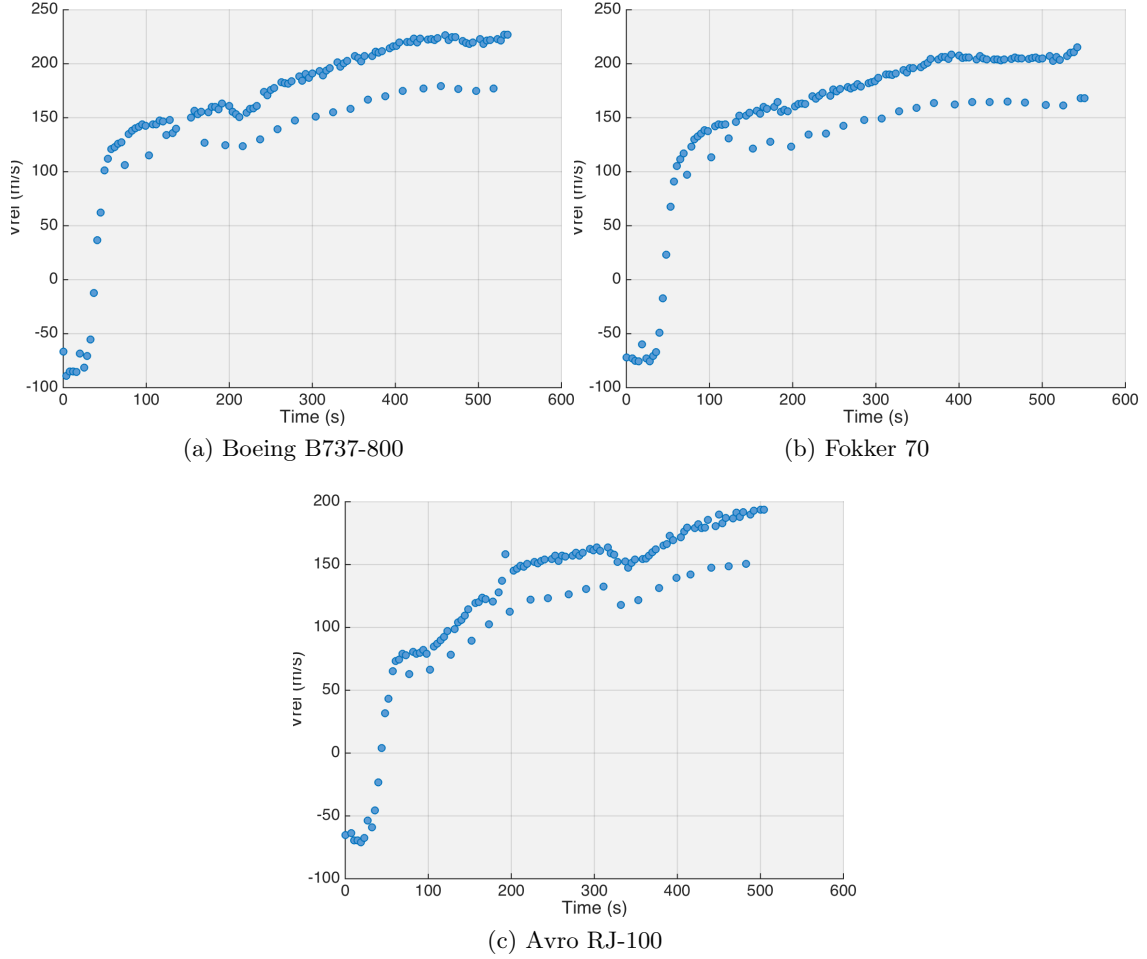
Figure 4.8: Relative velocity between different aircraft and NOMOS station 10
