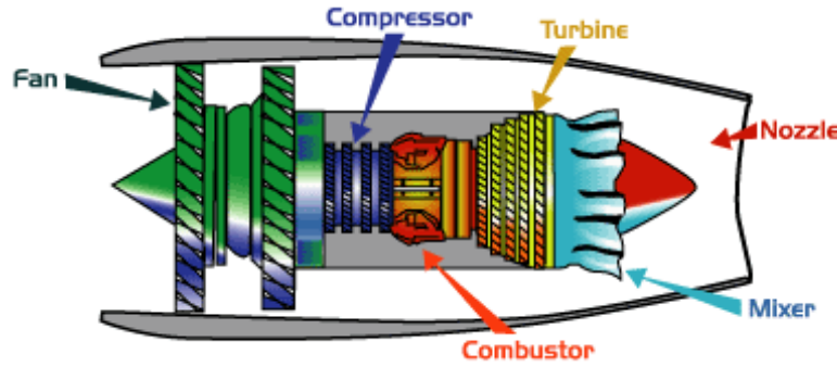
Figure 4.3: Schematic diagram illustrating the operation of a 2-spool, high-bypass turbofan engine, with LP spool in green and HP spool in purple. Retrieved from Ref. [31]
