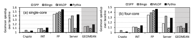
Figure 12: Performance on unseen traces.
