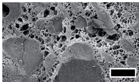
FIGURE 10: cryo-SEM image of bigel sample having 60 wt% of organogel captured after sublimation of water (scale bar = 10 μm) [62] “Reproduced with permission, Copyright [2015], [The Royal Society of Chemistry]”
