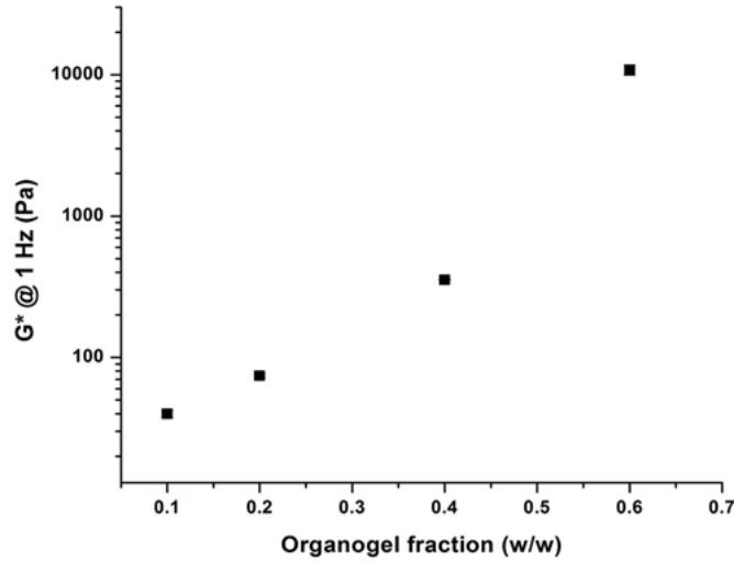
FIGURE 11: Complex modulus at 1 Hz as a function of organogel fraction for pectin/olive oil based bigels [63]
