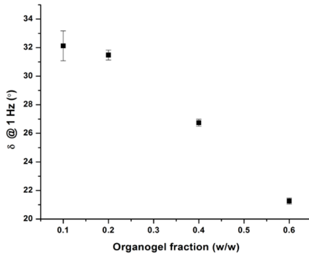
FIGURE 12: Phase angle at 1 Hz as a function of organogel fraction for pectin/olive oil based bigels [63]
