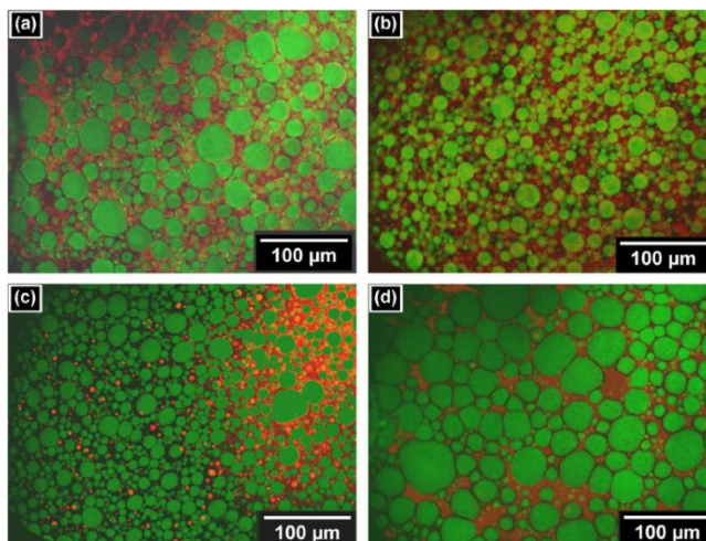
FIGURE 9: Fluorescent micrographs: (a) sodium alginate based bigels (b) sodium carboxy methyl cellulose based bigels (c) maltodextrin based bigels (d) starch based bigels [49], “Reproduced with permission, Copyright [2014], [John Wiley and Sons]”
