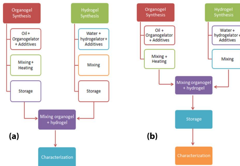
FIGURE 2: Block flow diagram for synthesis of bigels (a) by storing individual gels before bigel preparation and characterization (b) by mixing individual phases and then storing bigel formulations before characterization
