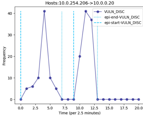
Fig. 3. Bursts of alerts from the same attack stage are aggregated into episodes. Here, an attack sequence related to vulnerability scanning is aggregated into two episodes.
