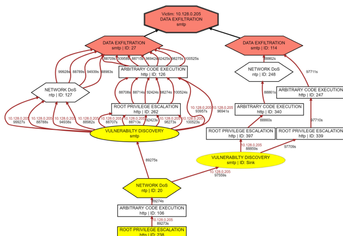
Fig. 12. Attack graph of data exfiltration over smtp for CCDC-2018. The same attacker host makes 13 attempts. Paths starting from severe attack stages are possible because the attack graphs show part of a full attack campaign.
