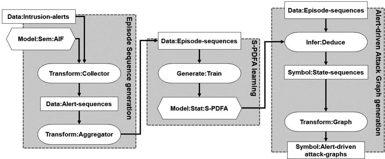
Fig. 1. SAGE takes intrusion alerts as input and generates attack graphs. Intrusion alerts are transformed into episode sequences (Section 4.1). An interpretable S-PDFA model is learned from those sequences (Section 4.2). The sequences are replayed through the S-PDFA and transformed into targeted attack graphs (Section 4.3).
