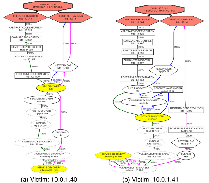
Fig. 11. Similar attacks targeting multiple victim hosts result in overlapping attack graphs.
