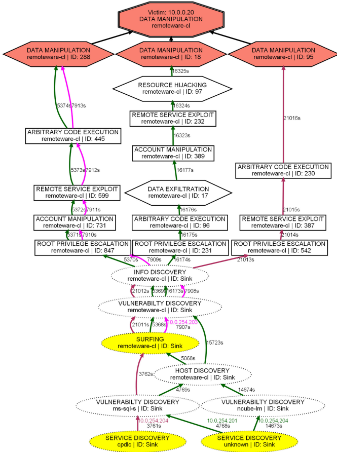
Fig. 9. An attack graph of data manipulation is a partial sub-graph of Fig. 8 because of overlapping attack paths.
