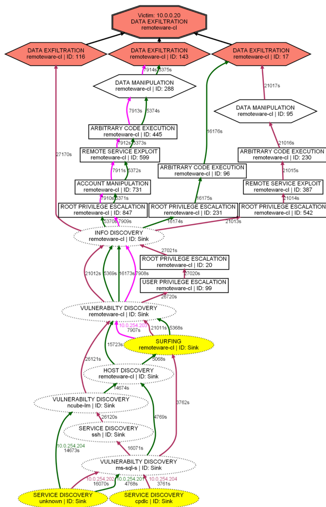
Fig. 8. Attack graph of data exfiltration over remoteware-cl. Three attacker teams successfully exploit it: Teams 1 and 5 exploit it twice, and each subsequent attempt is shorter than the first. The S-PDFA identifies three ways of exploiting the objective based on the actions that lead up to it.
