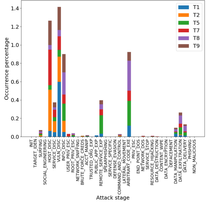
Fig. 2. The distribution of alerts per attack stage for the CPTC-2018 teams. Scanning-alerts are significantly more frequent than exploitation-alerts.
