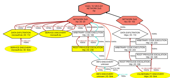
Fig. 13. Attack graph of network DoS over ntp for CCDC-2018. There are six possible starting actions and two possible ways to reach the objective.
