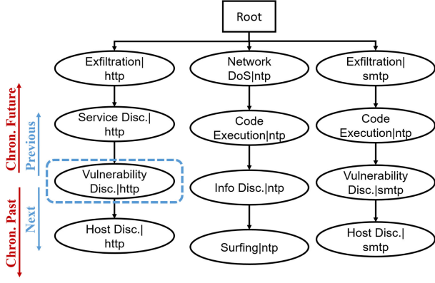
Fig. 5. A suffix tree for three traces. For any vertex, the previous vertex happens chronologically in the future.
