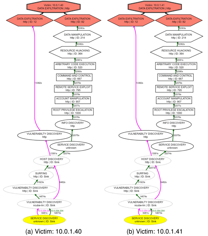
Fig. 10. Identical and simultaneous attacks targeting multiple victim hosts result in identical attack graphs.
