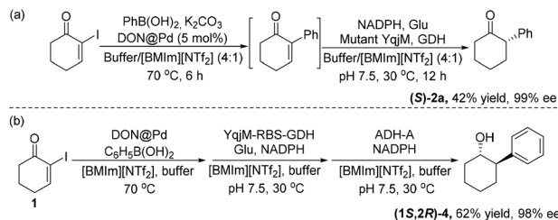
Scheme 3 (a) Chemoenzymatic asymmetric synthesis of (S)-2a and (b) three-step one-pot chemoenzymatic asymmetric synthesis of chiral \alpha -aryl cycloalkanol.
