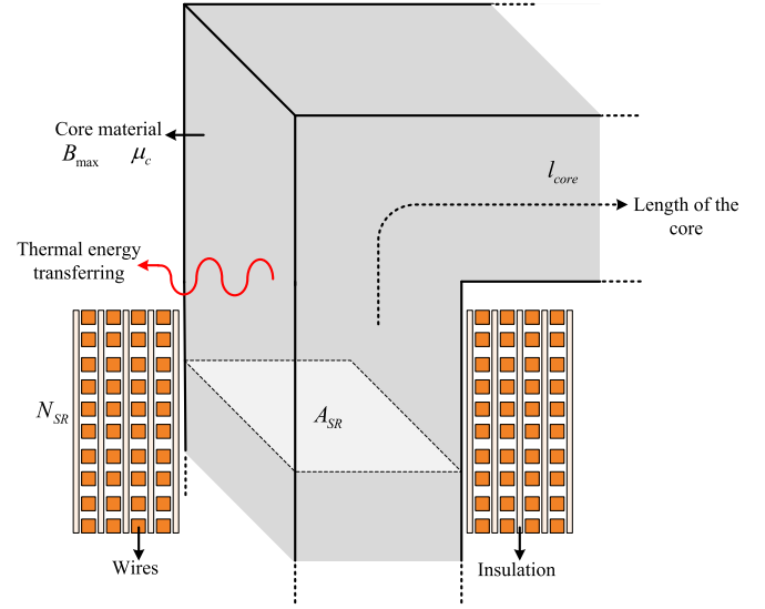
Fig. 6. Magnetic parameters of the magnetically coupled SR.
