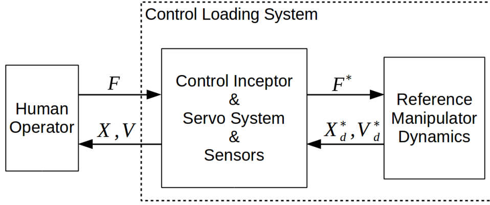
Figure 1: General structure of the control loading system with an admittance causality. Here, F denotes the force that a pilot applies on the control inceptor, X and V are the angular displacement and velocity of the inceptor. Superscript “*” denotes the discrete signals.
