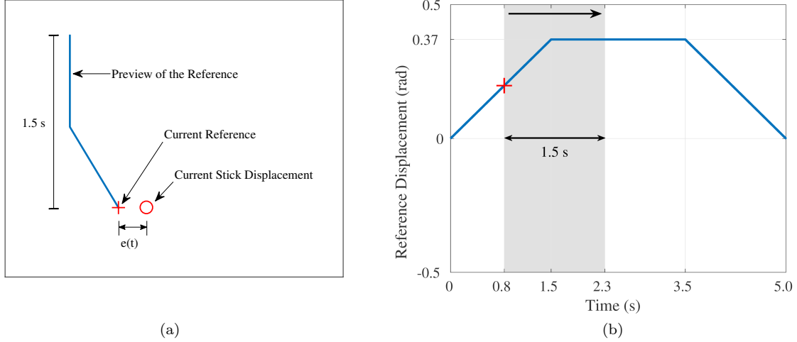
Figure 5: The visual display (a) and the trajectory of the target side-stick displacement (b) in the force-condition experiment.
