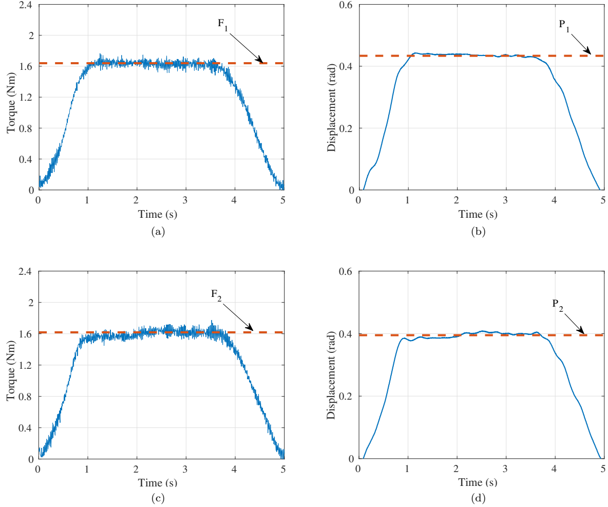
Figure 6: Side-stick forces and displacements applied by a subject in one trial in the free condition. F and P are obtained as the average of the stationary region, as shown by the red dashed lines.
