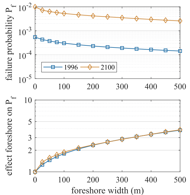
Fig. 12. Variation with foreshore width of (1) the failure probability in 1996 and (after sea level rise) in 2100 (top panel), and (2) the factor with which P_f decreases with respect to a 'dike only' system (bottom panel).
