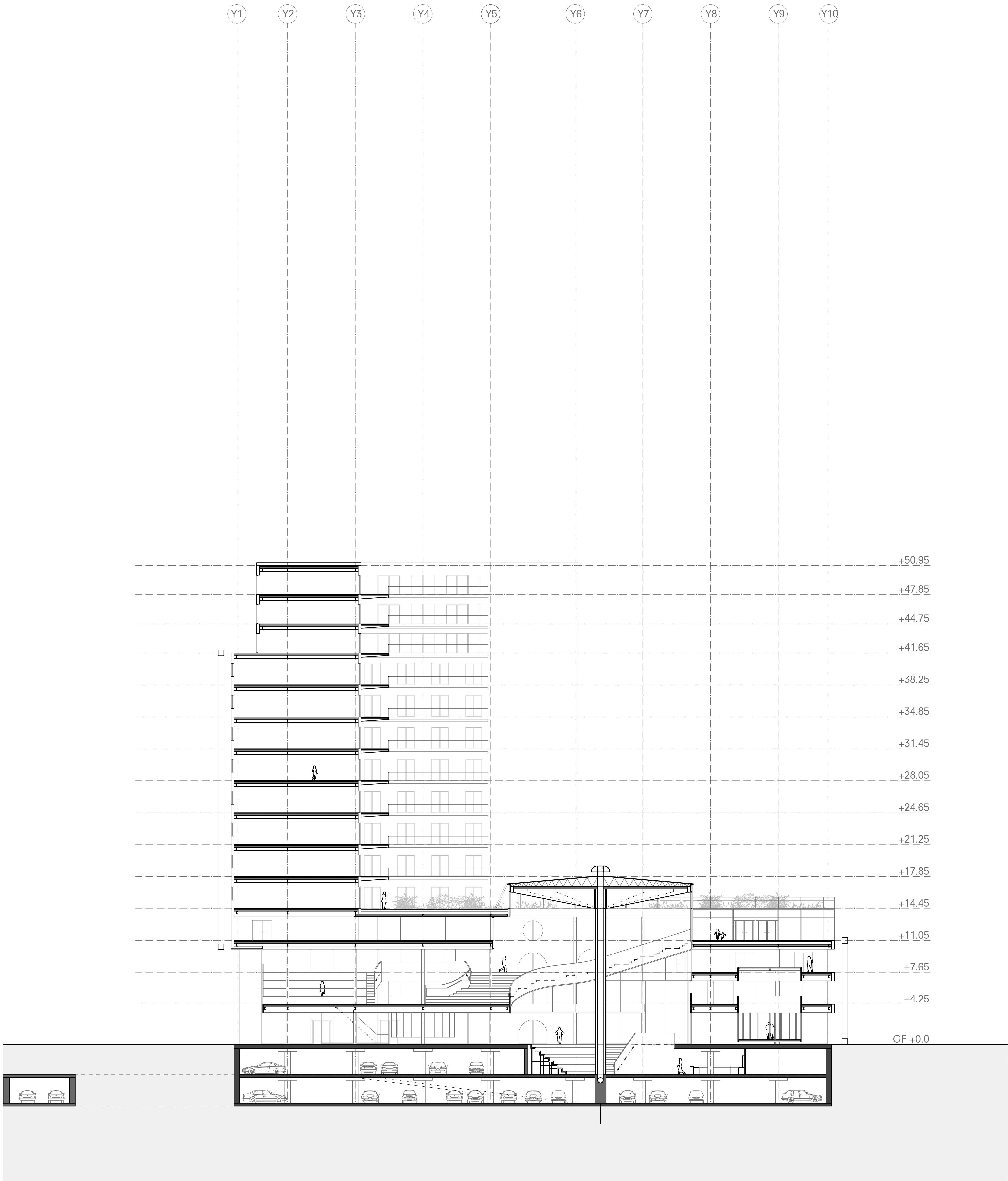
SECTION C-C 1:200
