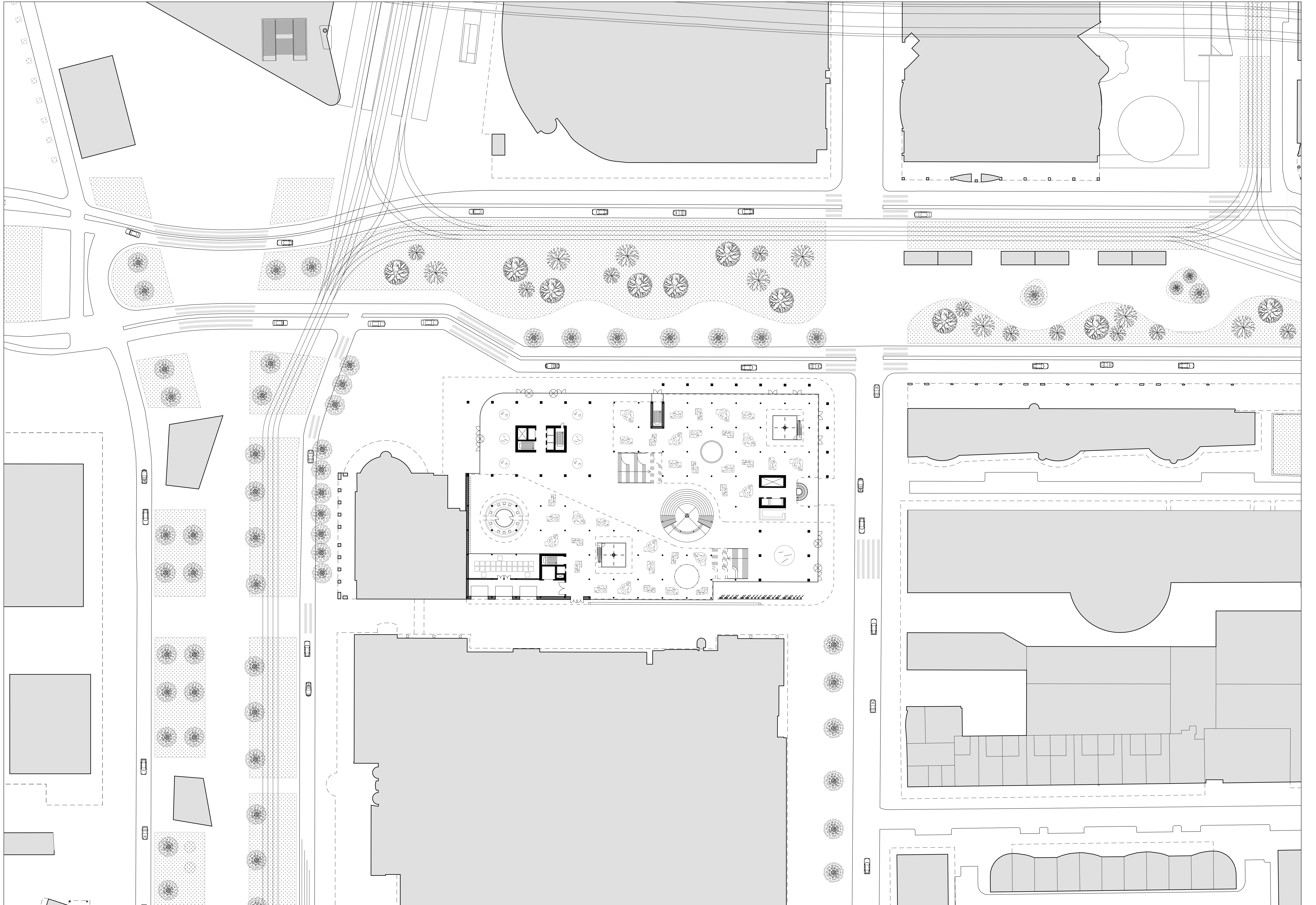
IMPLEMENTATION PLAN 1:1000
