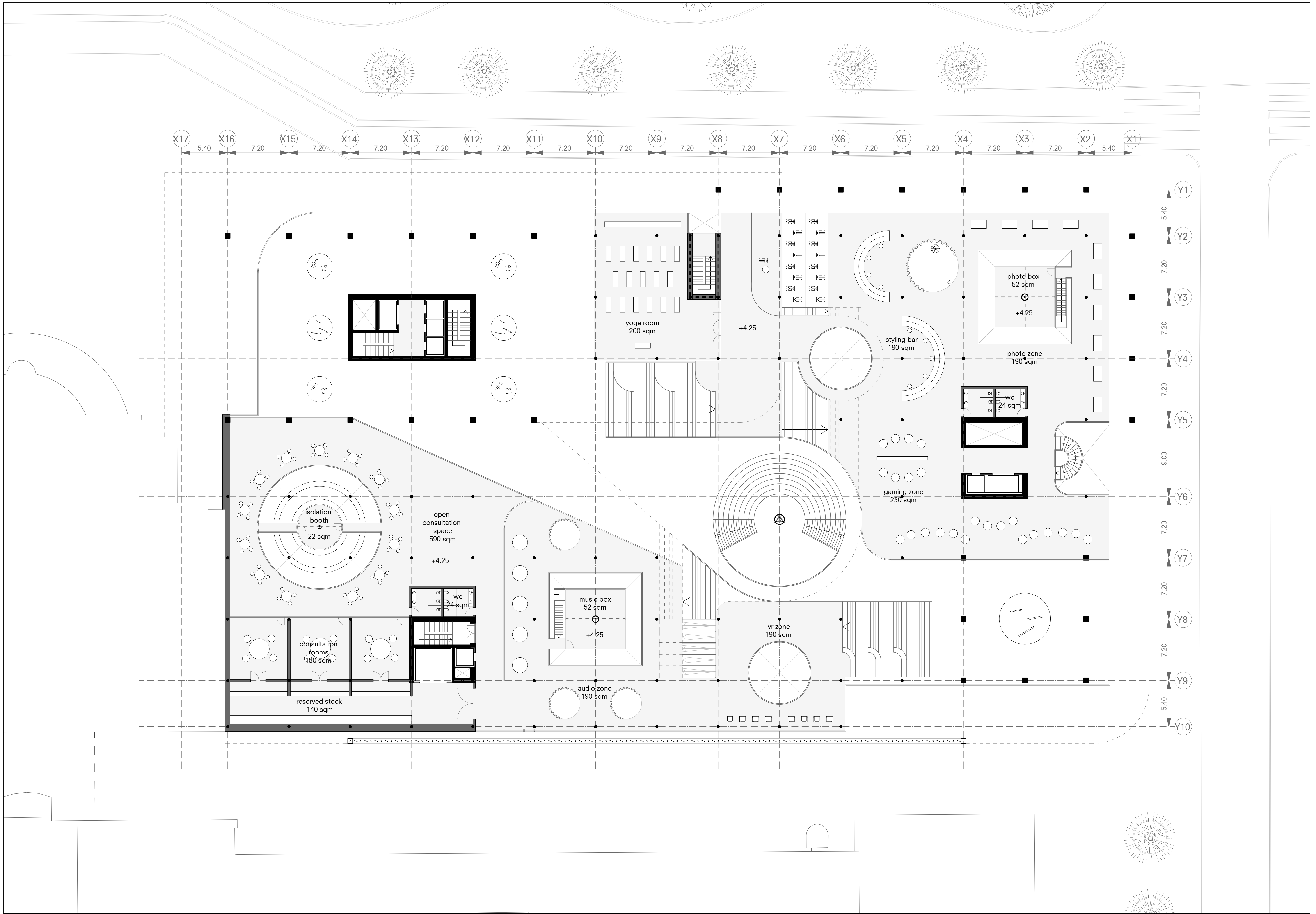
FLOOR 1 1:200
