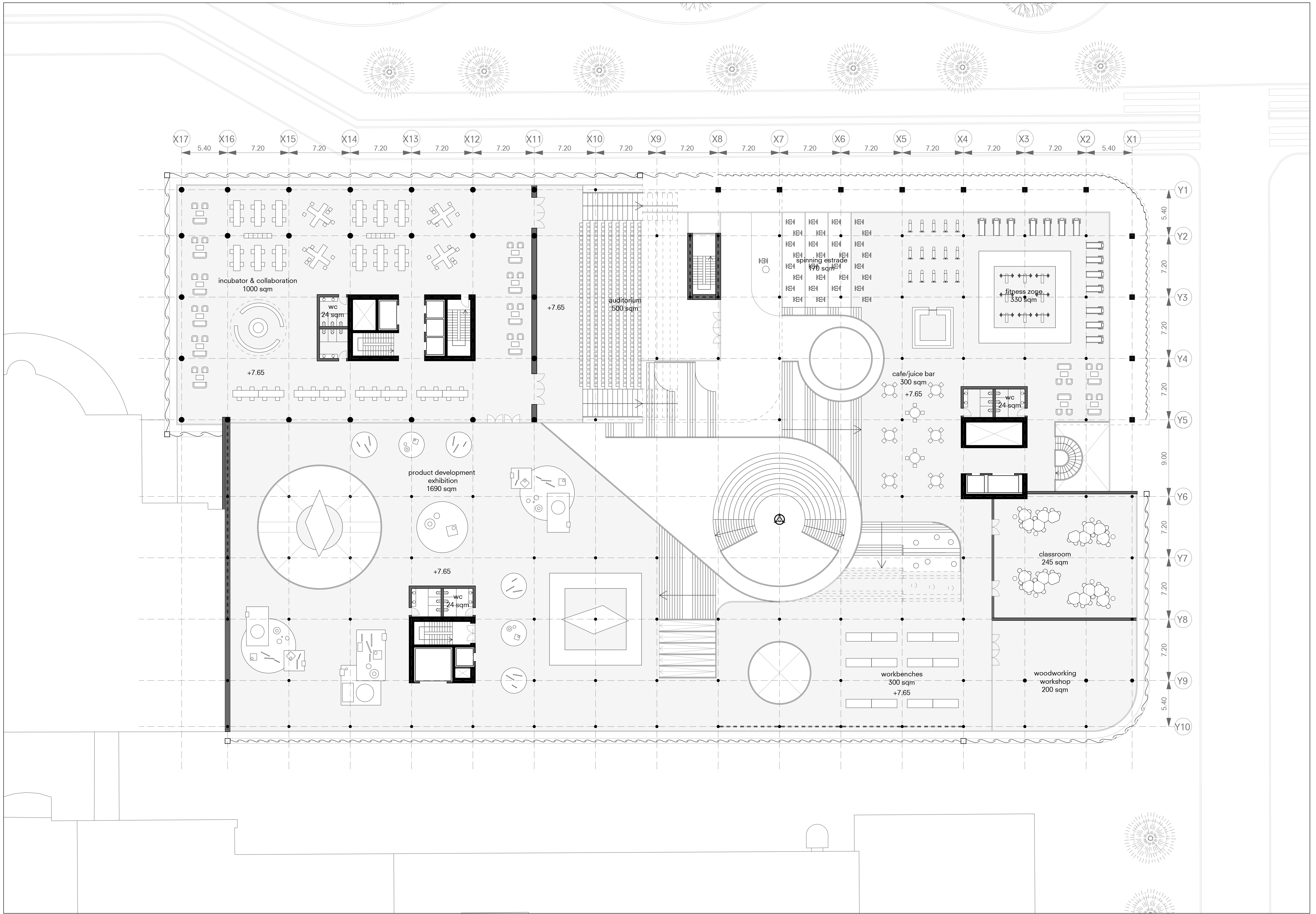
FLOOR 2 1:200
