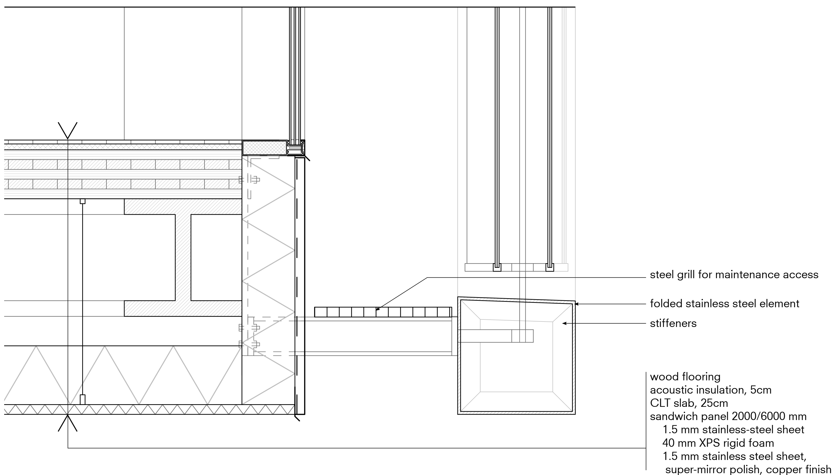
WALL DETAILS 1:10
