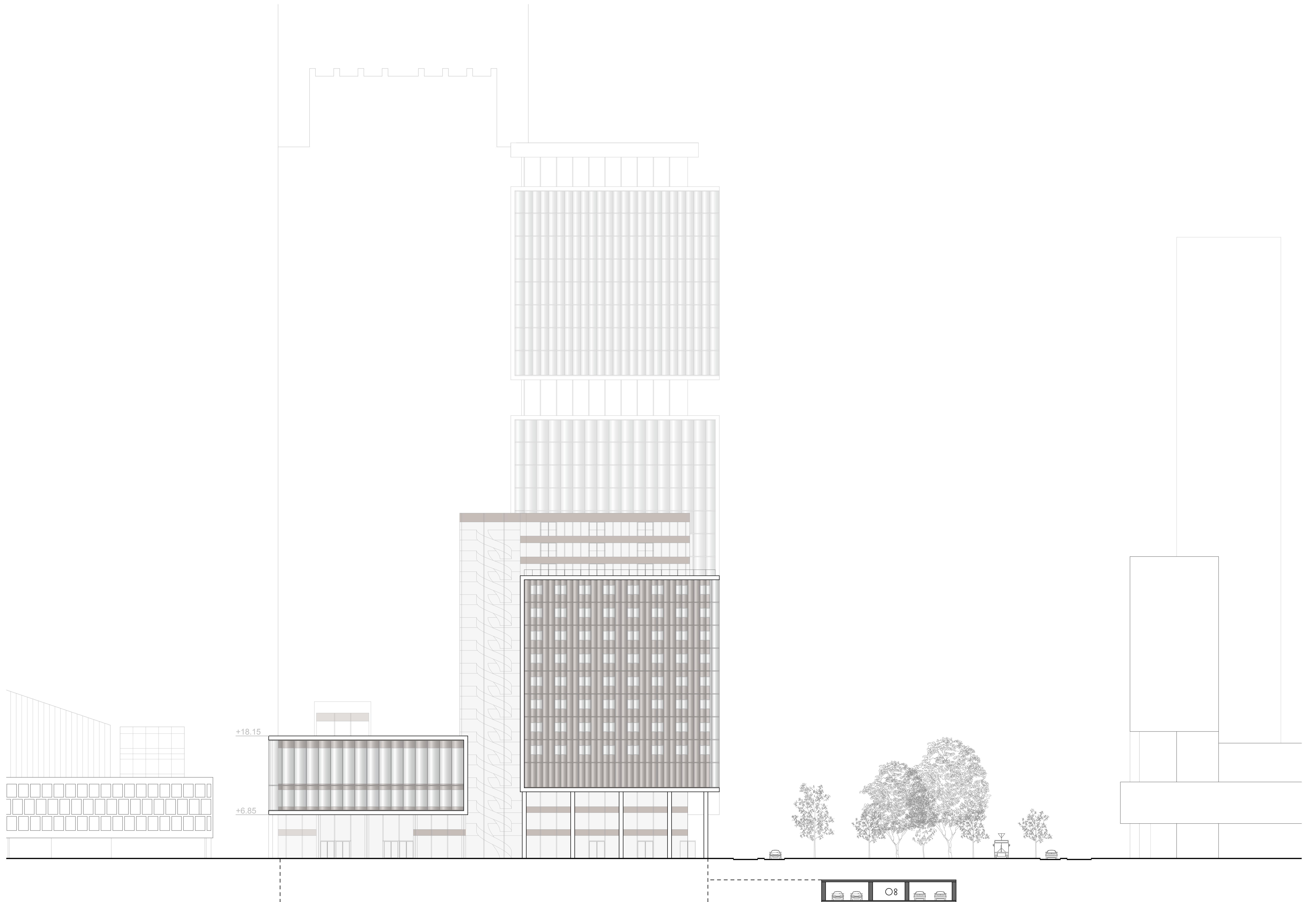
EAST ELEVATION 1:250
