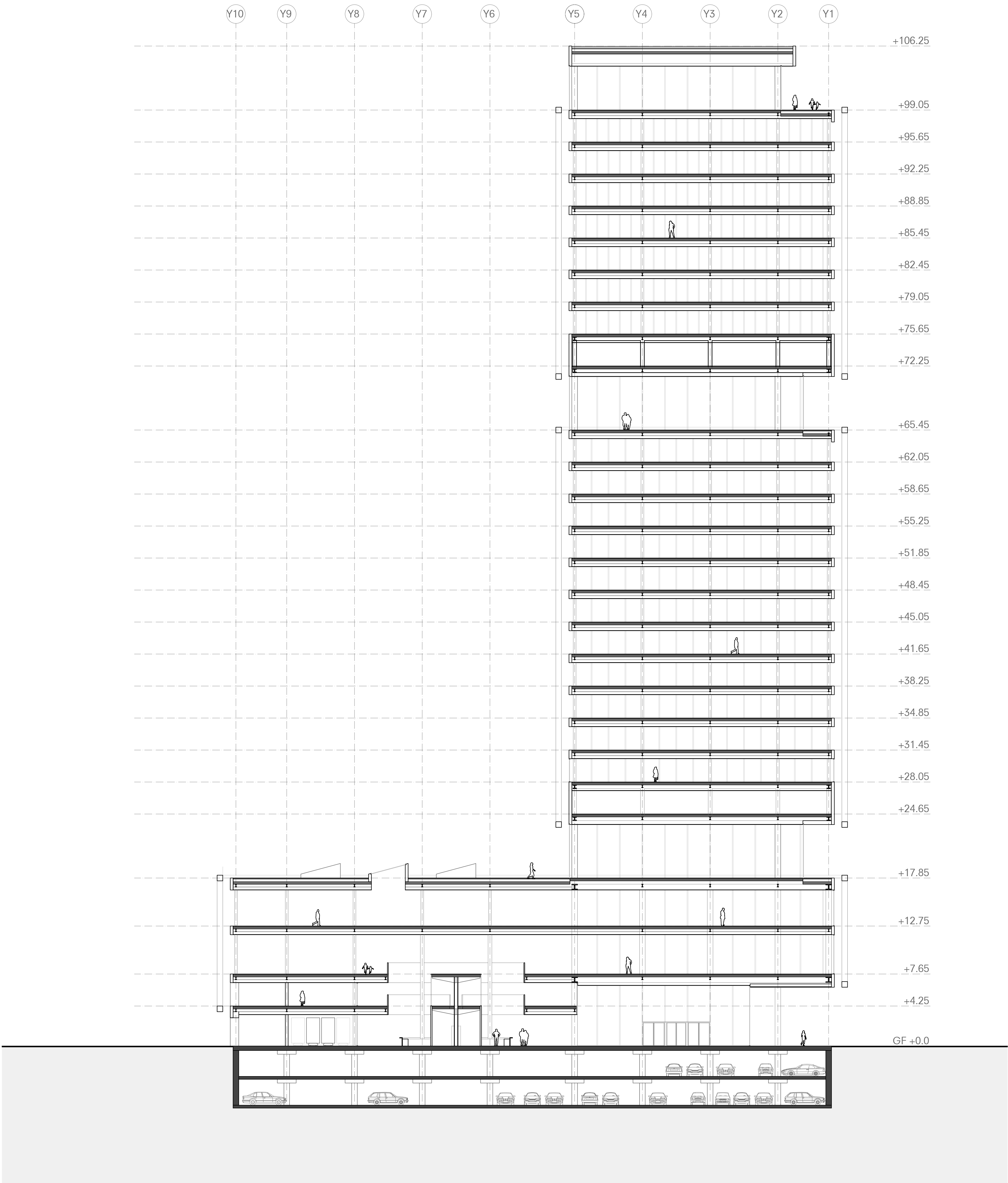
SECTION B-B 1:200
