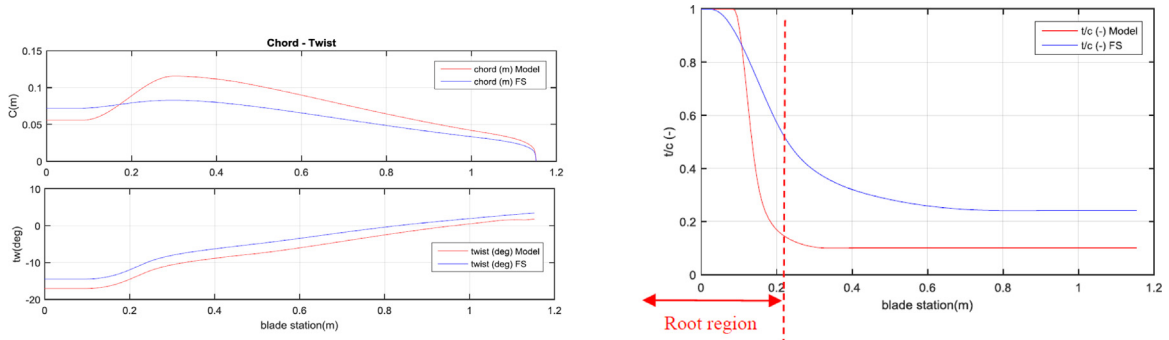
Fig. 2. Chord, twist and thickness distributions for the full scale DTU 10 MW (FS) and for the scaled model.
