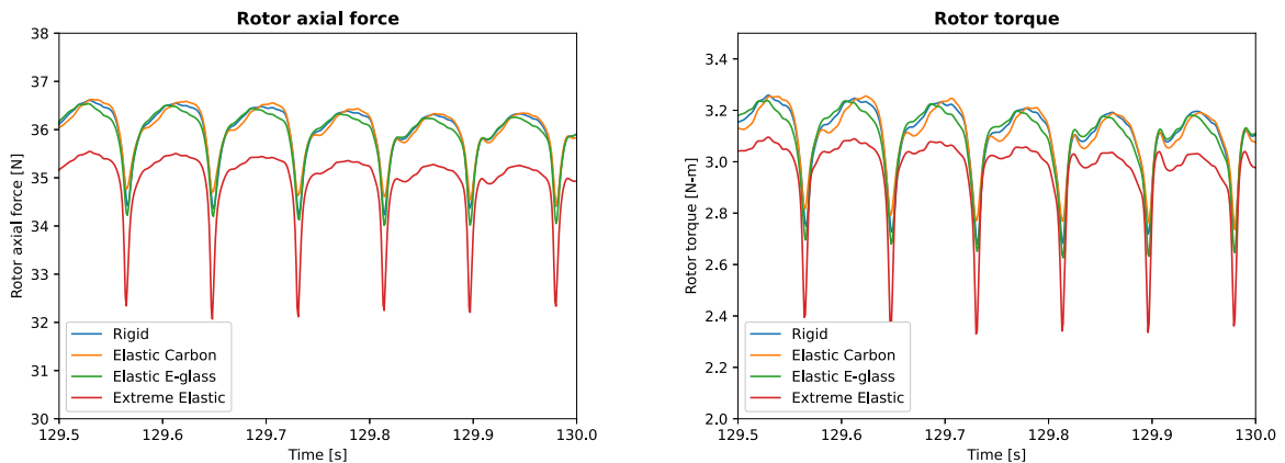
Fig. 11. Rotor performances - Below rated condition.
