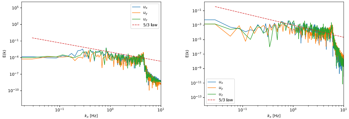
Fig. 7. Energy spectrum at (x, y, z) = (0, 0, 0) , rated (on the left) and above rated (on the right) conditions.
