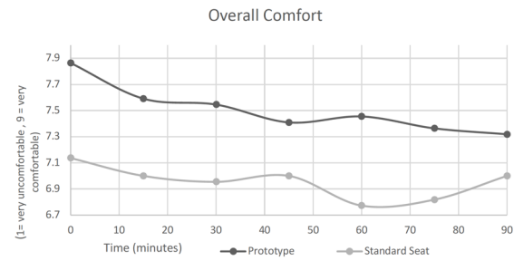
Fig. 13. Mean comfort rating of standard and prototype seat-pan against time ( n = 22 ).
