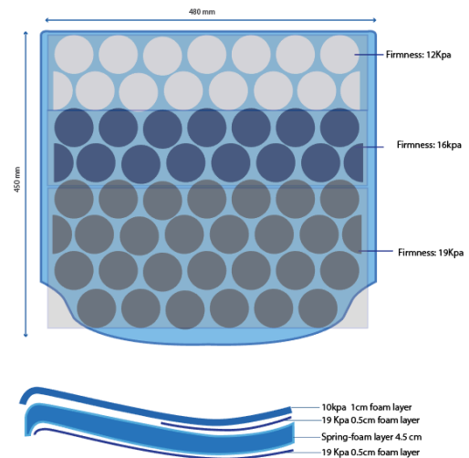
Fig. 18. Design for final iteration.
