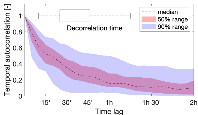
Figure 3. Temporal autocorrelation of the precipitation time series for the 133 debris-flow triggering events. Red and blue shaded areas show the 50 % and 90 % ranges across the 133 debris flow triggering events. The horizontal boxplot shows the distribution of the decorrelation times, calculated as the lag time at which the autocorrelation drops below e^{-1} .
