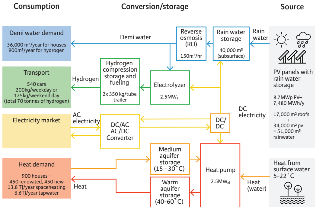
Figure 2.7 Schematic overview of the Power-to-H 3 system with supply, demand and system component sizes for the case of Nieuwegein, the Netherlands.
