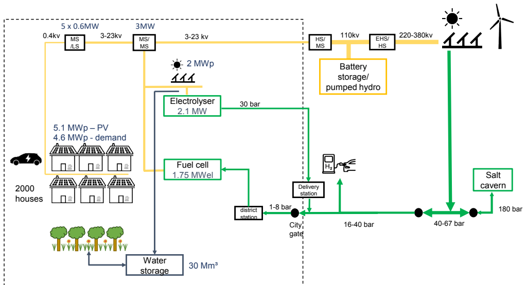
Figure 3.4 Schematic overview of the all-electric H 2 scenario that includes both an electrolyzer and fuel cell for local hydrogen production and uses while preventing grid reinforcement. The electricity supply by PV and electricity
