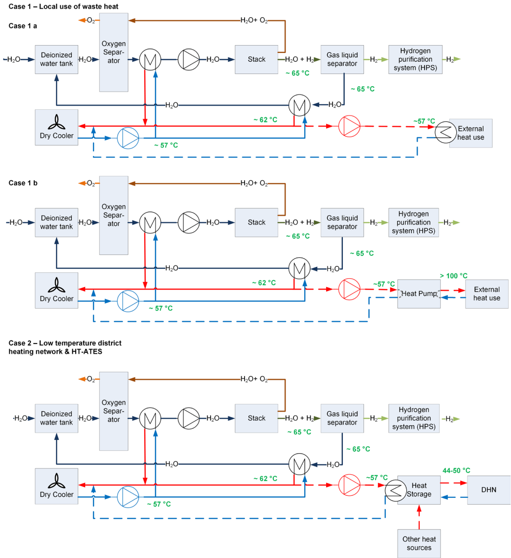
Figure 5.4 Redundant designs for heat recovery from a PEM electrolyzer.
