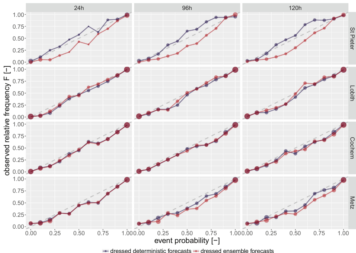
Fig. 9. Reliability plots for various lead times (columns) for several locations (rows). The plot is conditional on the observation exceeding the 50th percentile of the climatological exceedance probability (i.e., P = 0.50 ).
