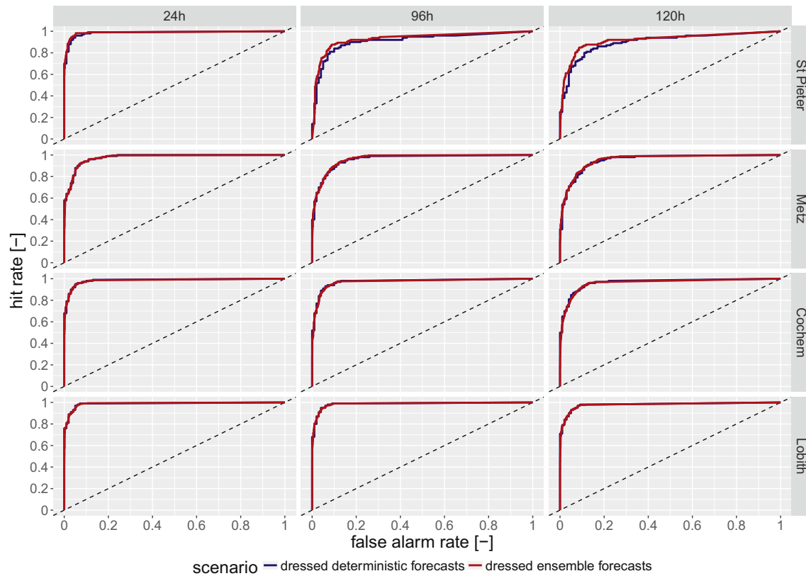
Fig. 15. ROC plots for various lead times (columns) for several locations (rows). The plot is for the event that the posterior water level exceeds the 90th percentile of the climatological exceedence probability (i.e., P = 0.90 ). The shading shows the width of the intervals obtained by bootstrapping the verification metric (see Section 2.7 for details).
