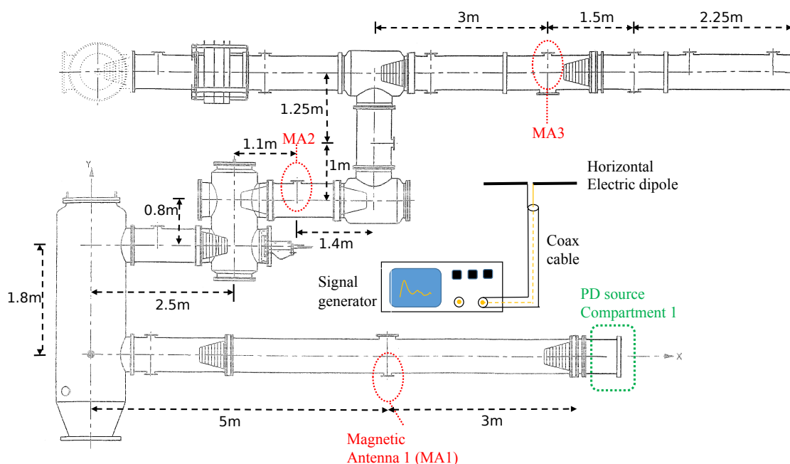
Figure 4. Test setup.
