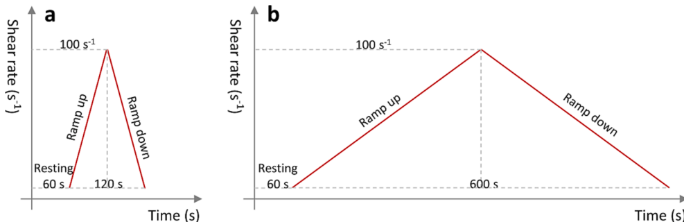
Fig. 2. Flow charts of (a) short cycle test and (b) long cycle test.
