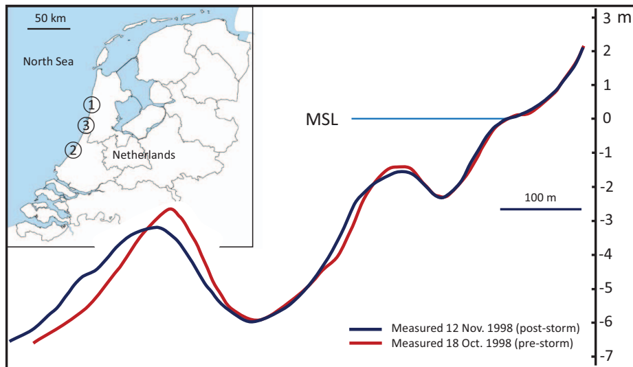
FIG. 8.—Change in average coastal profile at Egmond, Dutch coastal barrier, during a series of three successive storms. The average is based on 10 transects with an alongshore spacing of 100 m. Modified after Van Rijn et al. (2002). 1 Egmond; 2, Noordwijk; 3, Zandvoort.
