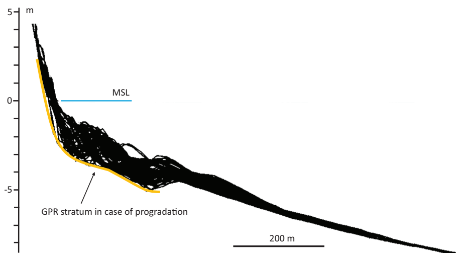
FIG. 6.—Sweep zone of 155 surveys of profile line 188 collected between 1981 and 1984 at Duck research facility, SC, USA. Modified after Birkemeier (1984).
