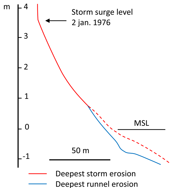
FIG. 5.—Deepest erosional scour of the Zandvoort beach, pole 70, Netherlands, between 2 Jan. 1968 and 6 Jan. 1978. Note that the analysis includes the storm of 2 Jan. 1976, one of the most severe storms of the century. Modified after Van den Berg (1977).
