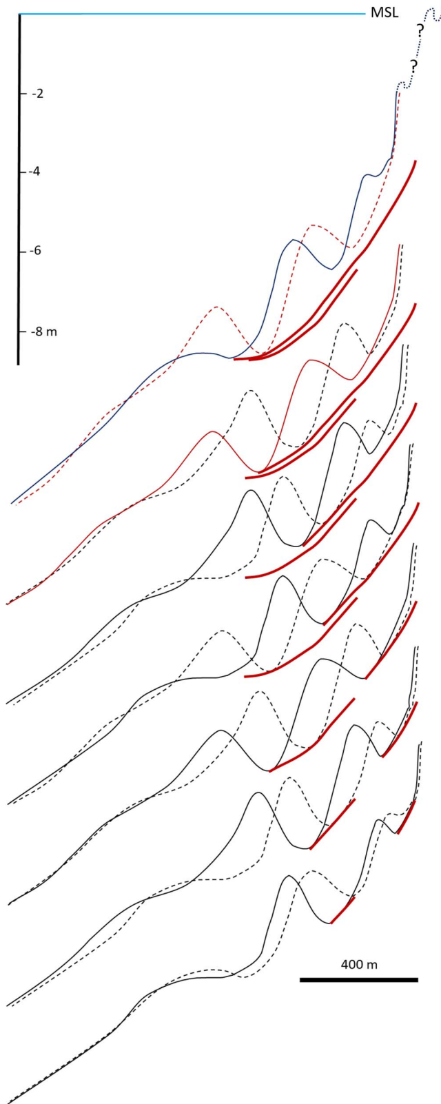
FIG. 4.—Longshore bar configurations in intervals of 3–6 months, depending on wave-energy conditions, at Long Beach Peninsula, based on model simulations (Cohn and Ruggiero 2016). The temporal succession is from base (oldest) to top (youngest). Dashed lines are former configuration, thick red lines are erosion surfaces.
