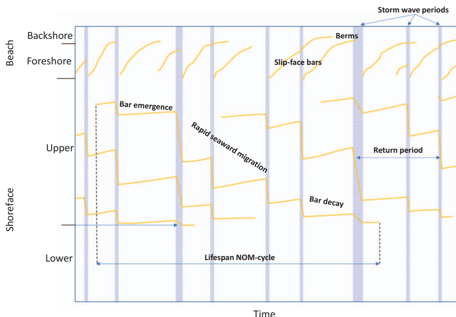
FIG. 3.—Parameters and terms used to define a NOM cycle. Bar-crest migration in the case of a longshore multi-bar system simplified by ignoring the influence of minor storms. Also indicated is the contrasting landward migration of foreshore slip-face bars that may eventually merge on backshore berms and their disappearance during extreme storm events. Based on Grunnet and Hoekstra (2004), Aleman et al. (2017), and short-term process understanding (Van Rijn et al. 2002; Masselink et al. 2006; Walstra et al. 2011; Walstra 2016; Walstra and Ruessink 2017).
