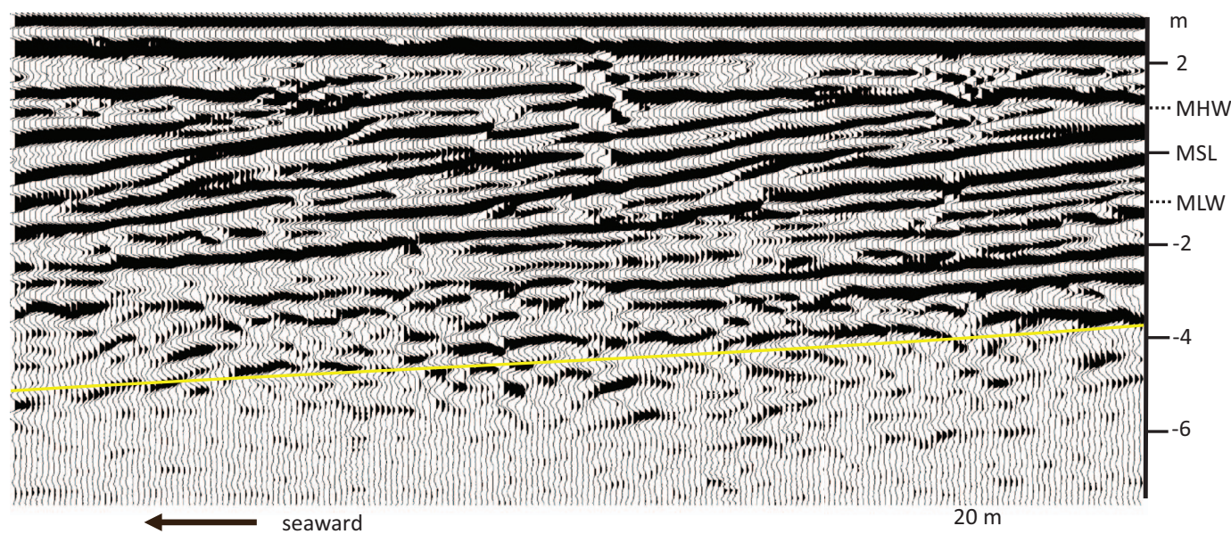
FIG. 1.—Cross-shore radargram (100 MHz) showing offshore inclined low-angle strata in less-than-a-century-old prograding coastal barrier deposits, Long Beach Peninsula, Washington, USA, modified after Jol et al. (2002). Surface elevation obtained from US Topographical Map. For location see Fig. 2. Yellow line shows agreement with scour line deduced from morphodynamic processes in the present-day shoreface (see Fig. 4). MSL, mean sea level; MHW, mean high water; MLW, mean low water.
