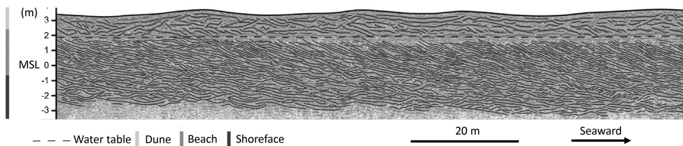
FIG. 7.—Cross-shore radargram (250 MHz) showing landward-climbing low-angle units downlapping on and sandwiched in between SIS, Boydtown barrier, SE Australia (Fig. 7F in Oliver et al. 2017).
