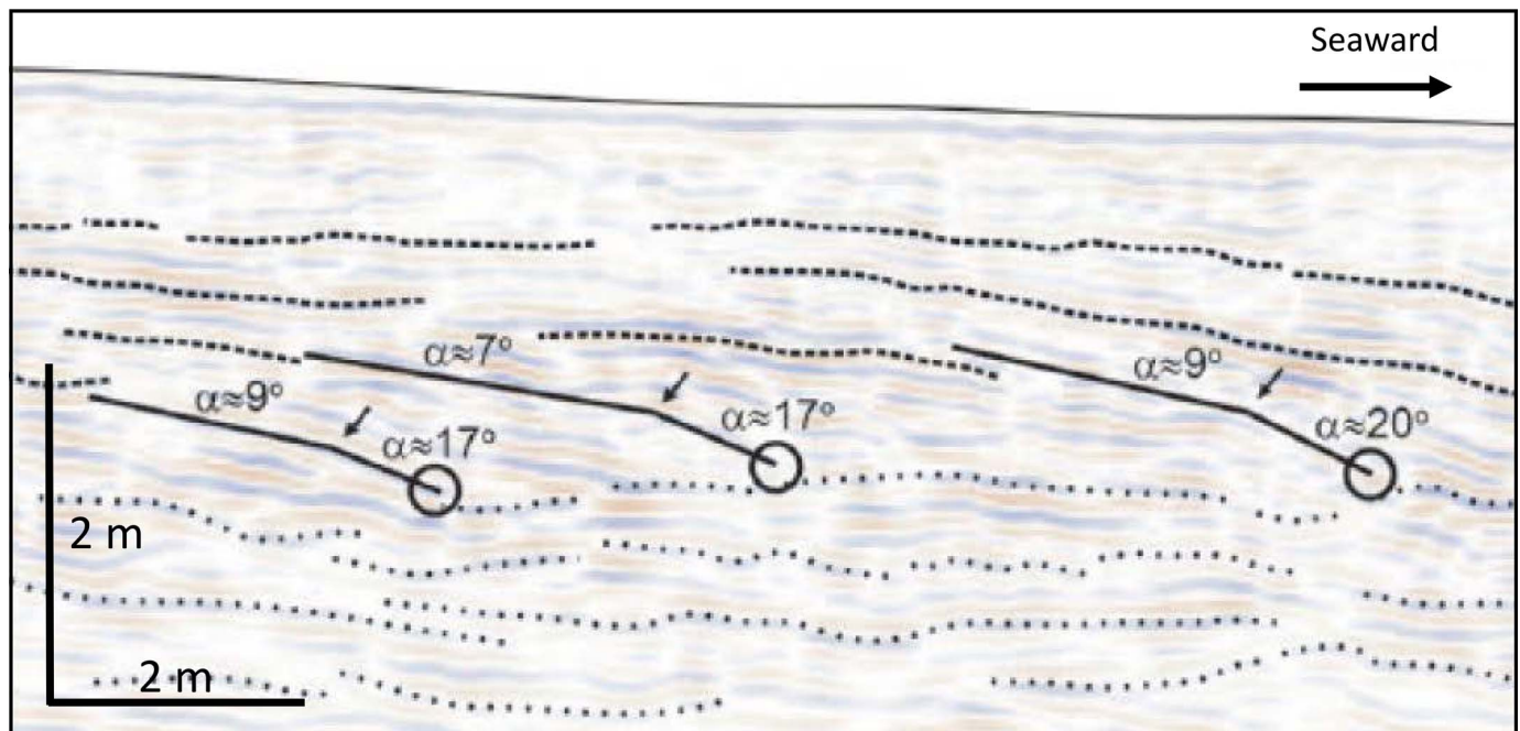
FIG. 10.—Example of GPR reflection data (250 MHz) with interpreted beach-face and upper-shoreface deposits. Raised beach-ridge system, Samsø, Kattegat Sea, Denmark. Note the occurrence of some kinks in the dip that mark the transition of the upper shoreface to the beach (marked by arrows). From Hede et al. (2015). DVR90, Danish Vertical Reference 1990.
