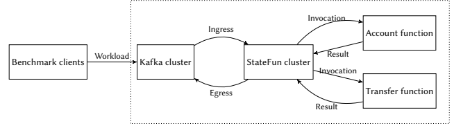
Figure 3: Benchmark application architecture
