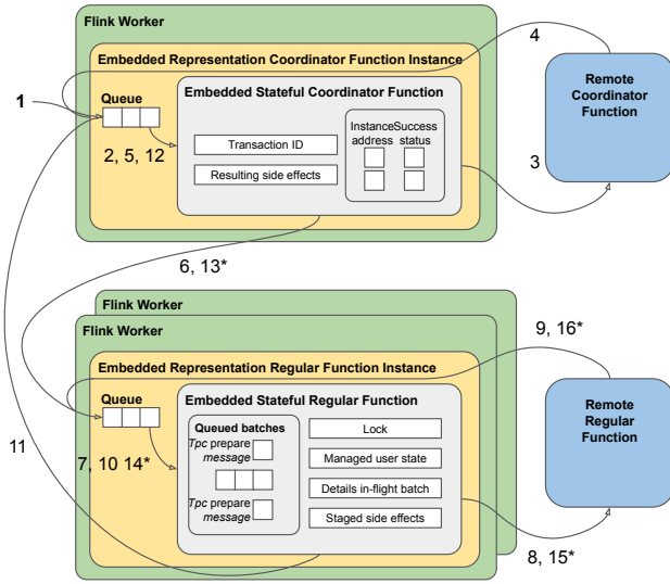
Figure 2: Communication flow for transactions.
