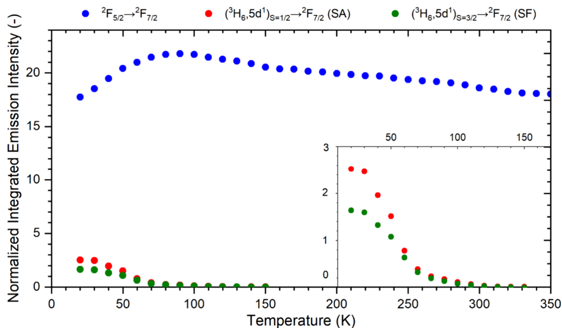
Figure 7. Plot showing the integrated emission intensity of the ^2\text{F}_{5/2} \rightarrow ^2\text{F}_{7/2} (blue), (^3\text{H}_6,5\text{d}^1)_{S=1/2} \rightarrow ^2\text{F}_{7/2} (red), and (^3\text{H}_6,5\text{d}^1)_{S=3/2} \rightarrow ^2\text{F}_{7/2} (green) emissions after excitation into the (^3\text{H}_6,5\text{d}^1)_{S=1/2} levels at 570 nm. The data is normalized and extrapolated on the measured ^2\text{F}_{5/2} \rightarrow ^2\text{F}_{7/2} quantum efficiency at 300 K and corrected for the sensitivity of detection. The inset shows a close-up of the 4\text{f}^{12}5\text{d}^1 \rightarrow 4\text{f}^{13} emissions.
