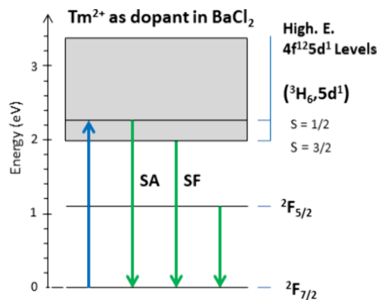
Figure 6. Scaled energy level scheme for \text{Tm}^{2+} as a dopant in \text{BaCl}_2 with an orthorhombic structure. Upon excitation into the low-spin (^3\text{H}_6,5\text{d}^1)_{S=1/2} levels (blue arrow) at 20 K, three distinct \text{Tm}^{2+} emissions are observed (green arrows). Note: SA = spin-allowed; SF = spin-forbidden.
