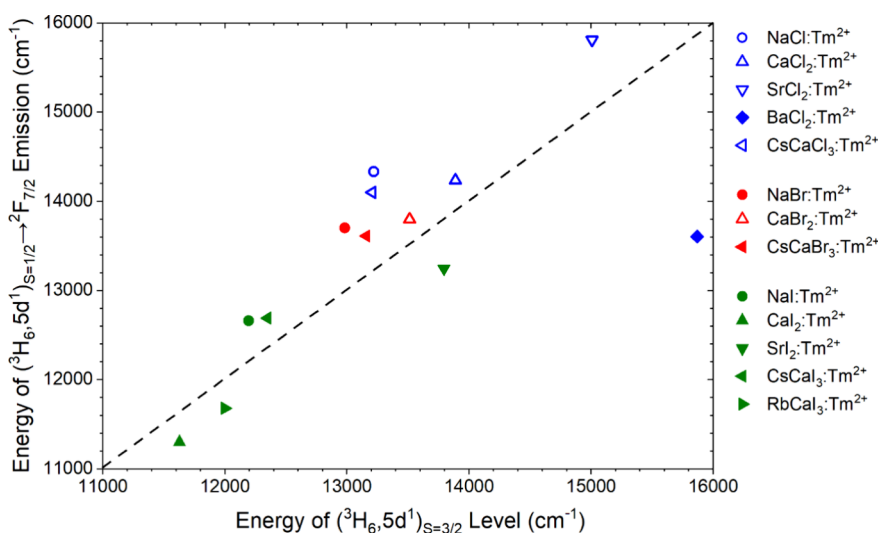
Figure 9. Graph showing the absorption energy of the (^3H_6,5d^1)_{S=3/2} levels plotted versus the luminescence energy of the (^3H_6,5d^1)_{S=1/2} \rightarrow ^2F_{7/2} emission for all previously studied Tm^{2+} -doped halides, excluding fluorides. 19,21,24–27 The closed symbols represent compounds in which the (^3H_6,5d^1)_{S=1/2} \rightarrow ^2F_{7/2} emission was perceived, while for the open symbols, this emission was not observed, but its presumed energy was calculated from the 4f^{12}5d^1 Stokes shift. The (^3H_6,5d^1)_{S=1/2} \rightarrow ^2F_{7/2} emission has a relatively strong luminescence signature in compounds, where its energy is lower than the (^3H_6,5d^1)_{S=3/2} absorption energy. Note that the line serves as an aid to the eye.
