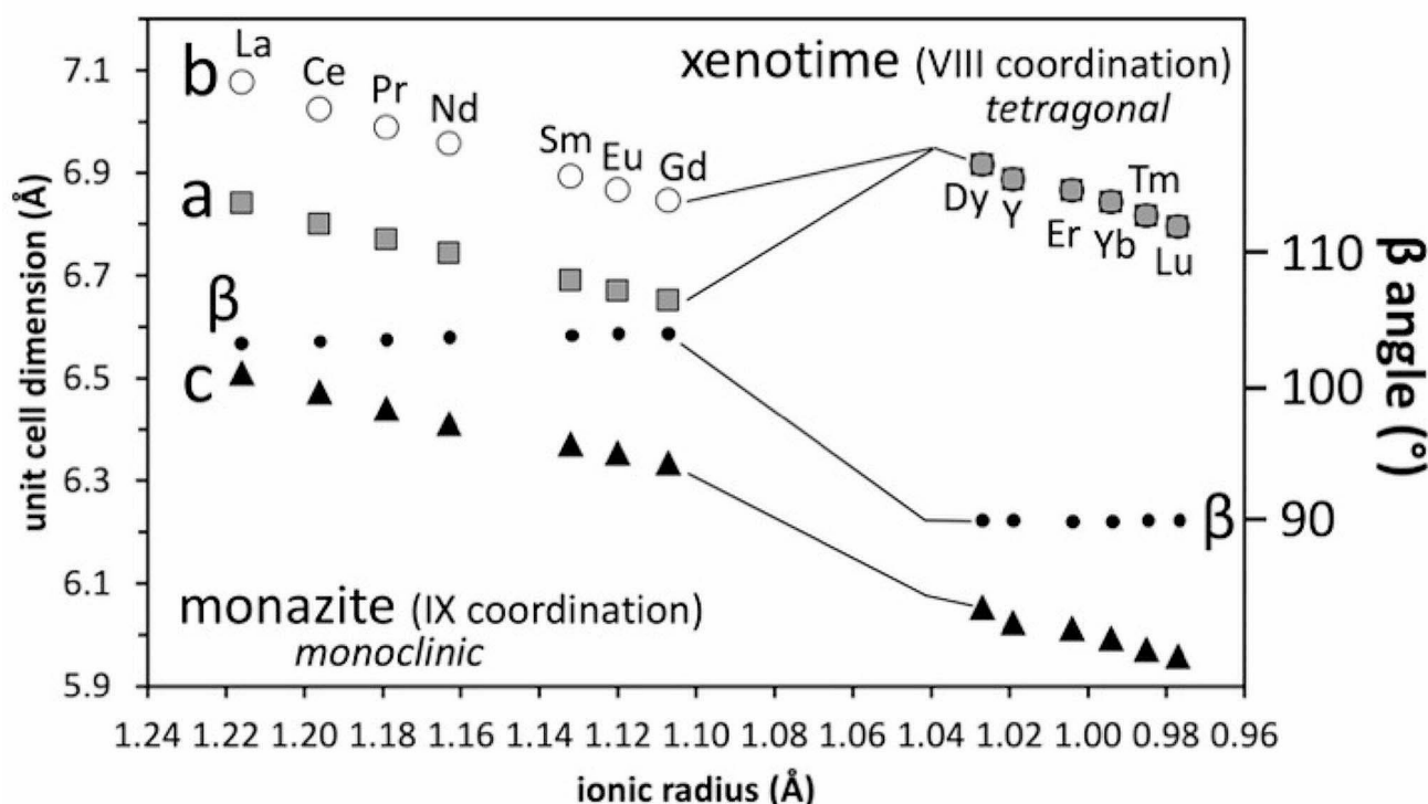
Fig. 4 Results of the structural refinement of the X-ray diffraction data of synthesized monazite and xenotime, showing the systematic decrease of unit cell dimensions a , b , c with decreasing ionic radius of the lanthanides from La to Lu (lanthanide contraction), and the switch
