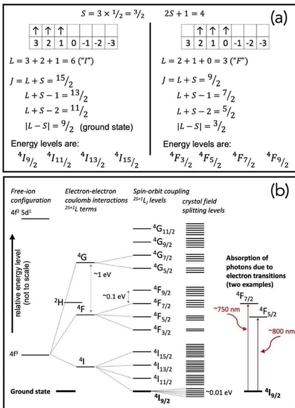
Fig. 2 (a) Two worked-out examples of Russell-Saunders notation of energy levels of the 4f electrons in the \text{Nd}^{3+} ion with configuration \{\text{Xe}\} 4f^3 . See also text for discussion. Both examples are cases with three electrons spinning up, as shown by the three upward pointing arrows (so S = 3/2 ), but with different orbital angular momenta ( L = 6 and L = 3 ), and different spin-orbit coupling levels J . The ^4I_{9/2} level is the one with the lowest energy, i.e., the ground state for the \text{Nd}^{3+} ion. (b) Schematic representation of the energy splitting effects due to coulomb-type electron-electron interactions ( ^{2S+1}L terms, i.e., ^4I , ^4F , ^2H , ^4G , ...), further splitting into ^{2S+1}L_J levels due to spin-orbit coupling ( ^2H and ^2K levels omitted for clarity, but see Fig. 9 for their positions), and further splitting into so-called Stark levels due to crystal field effects. Relative positions of ^{2S+1}L_J levels are based on data from Carnall et al. (1978); number of crystal field levels per ^{2S+1}L_J level are for non-cubic site symmetry (Eliseeva and Bünzli 2010). Energy levels are not to scale, but order-of-magnitude values of splitting energies (in eV) are indicated. Two electronic transitions, from the ground state ^4I_{9/2} to ^4F_{7/2} and ^4F_{5/2} are highlighted on the right; these can be achieved by absorption of photons with wavelengths of \sim 750 and \sim 800 nm respectively
