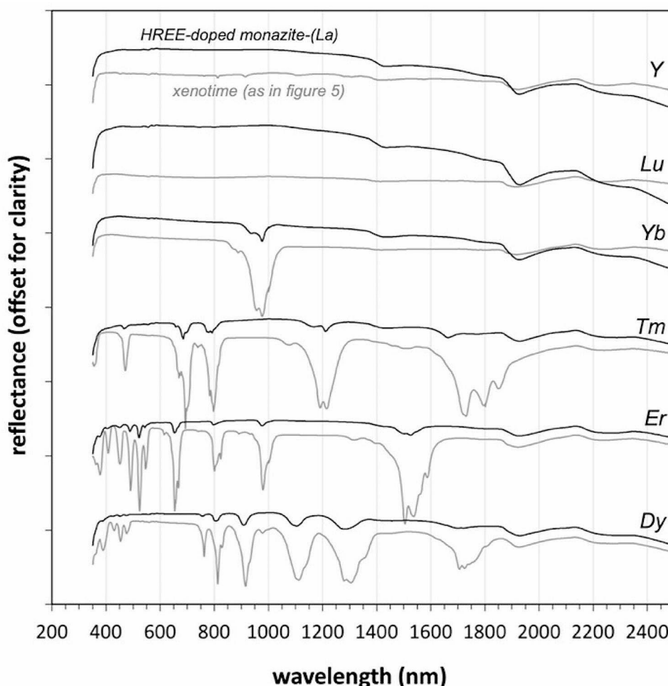
Fig. 6 Comparison between reflectance spectra of xenotime-(HREE) shown as grey curves, and monazite-(La) doped with the same REE (where molar HREE/(La + HREE) is c. 5%) shown as black curves. There is a strong effect of the much lower concentrations of the spectrally active HREE in the doped monazites, expressed as a reduced depth of the absorption features. The splitting of the absorption features into multiplets, corresponding to the Stark levels due to splitting of the energy levels under the influence of the crystal field, is also much more clearly expressed in the xenotime powders. It is also noteworthy that well-defined absorption features at wavelength > 1600 nm in the xenotimes of Dy and Tm are not observed in the corresponding Dy and Tm-doped monazites
