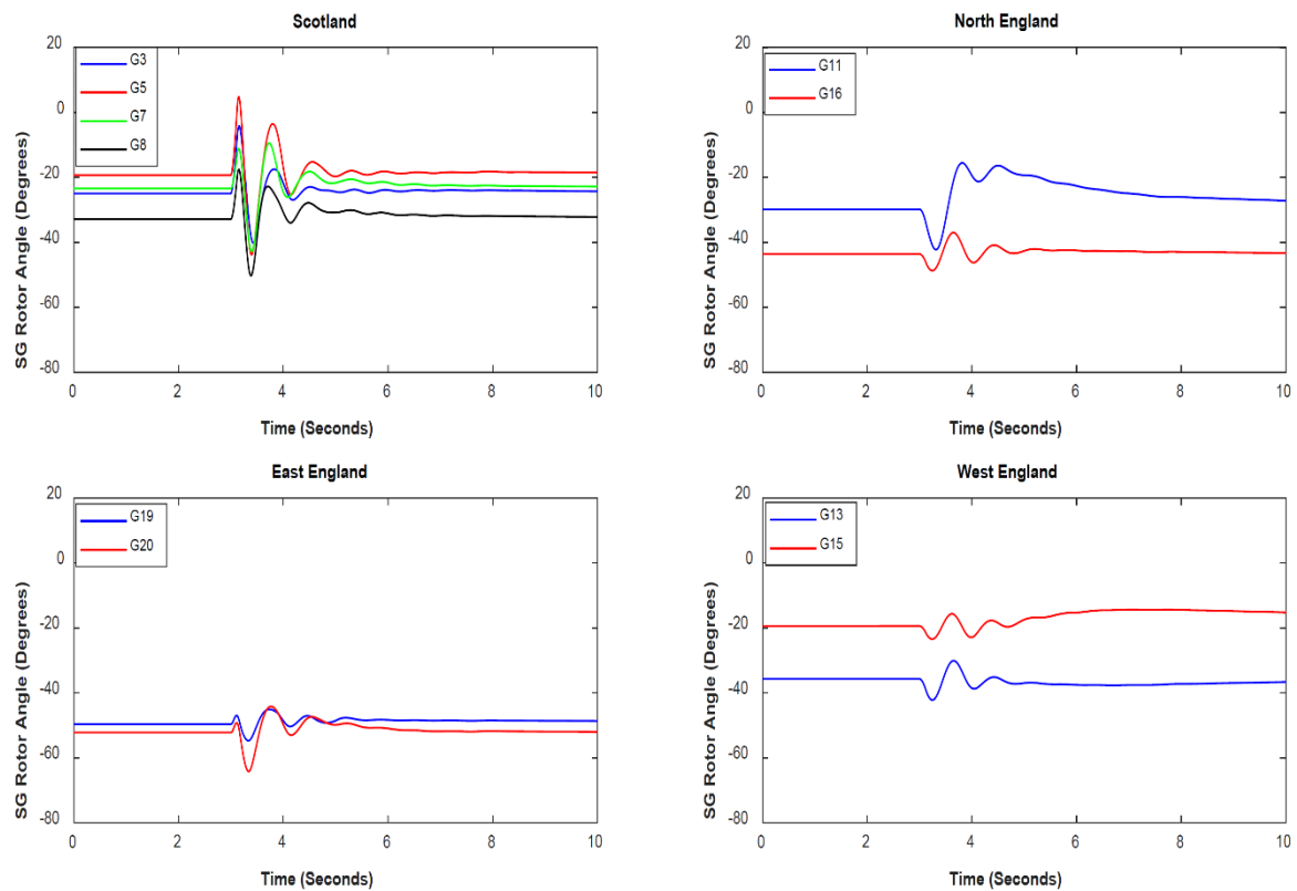
Figure 15. SGs' rotor angles' responses for a 120 ms three-phase fault at line 6–9 under a 66% share of wind generation in the GB system. Fault clearing time (FCT) = 120 ms. All WGs equipped with PAM controller.
