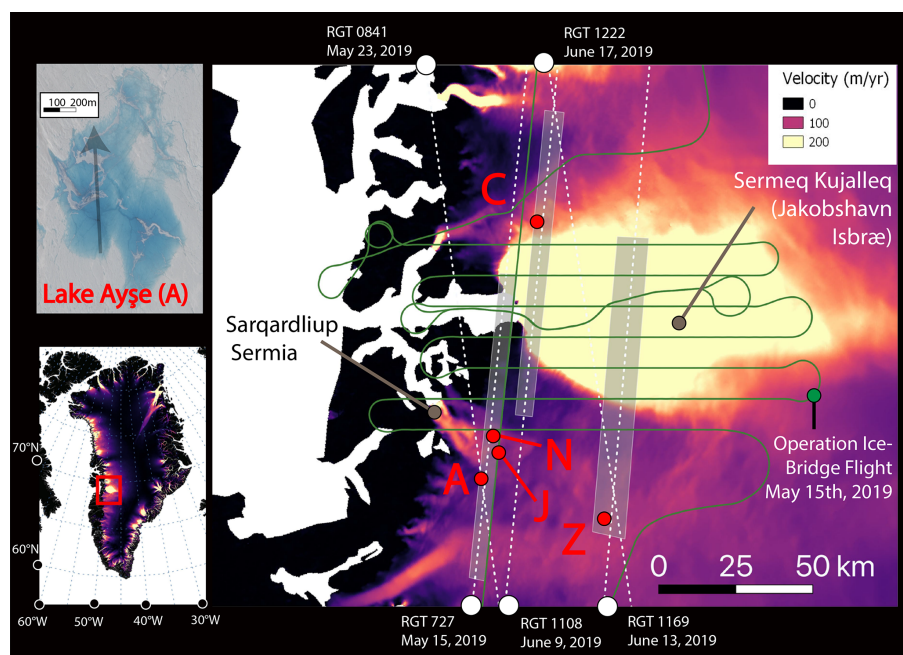
Figure 1. Study region over Sermeq Kujalleq and Sarqardliup Sermia. Top left panel: Lake Ayse on 23 May using Planet SkySat Visual imagery. Bottom left panel: study region over western Greenland. Right panel: main region with repeat-tasking locations for Planet SkySat shown in grey boxes over annual velocity estimates from MEaSUREs (NSIDC). ICESat-2 reference ground tracks shown in white. Operation IceBridge flight on 15 May 2019 shown in green. Five lakes indicated in red discussed throughout text include the following: C: Lake Cecily; A: Lake Ayse; J: Lake Julian; N: Lake Niels; Z: Lake Zadie.
