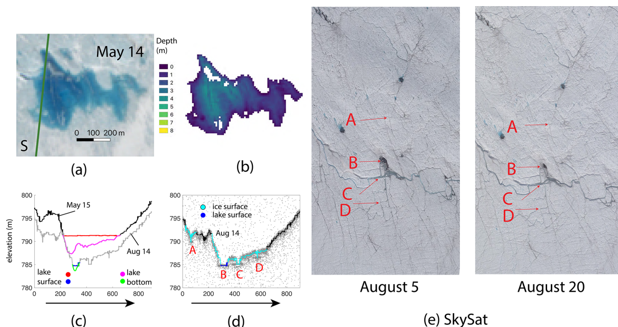
Figure 10. ICESat-2 RGT 727 over Lake Julian. (a) Sentinel-2-based imagery acquired on 14 May 2019 with ICESat-2 RGT 727 gt11 (occurring on 15 May and 14 August 2019) overlapping in green. Operation IceBridge overpass on 15 May 2019 is directly coincident with the ICESat-2 line. (b) Lake depth derived from Watta (c) and Sentinel-2 (a) imagery. (c) Watta calculated from ICESat-2 on 15 May and 14 August. (d) Watta-calculated surface features over photon cloud on 14 August. Points A–D discussed in text. (e) Points A–D shown over Planet SkySat imagery collected on 5 and 20 August.
