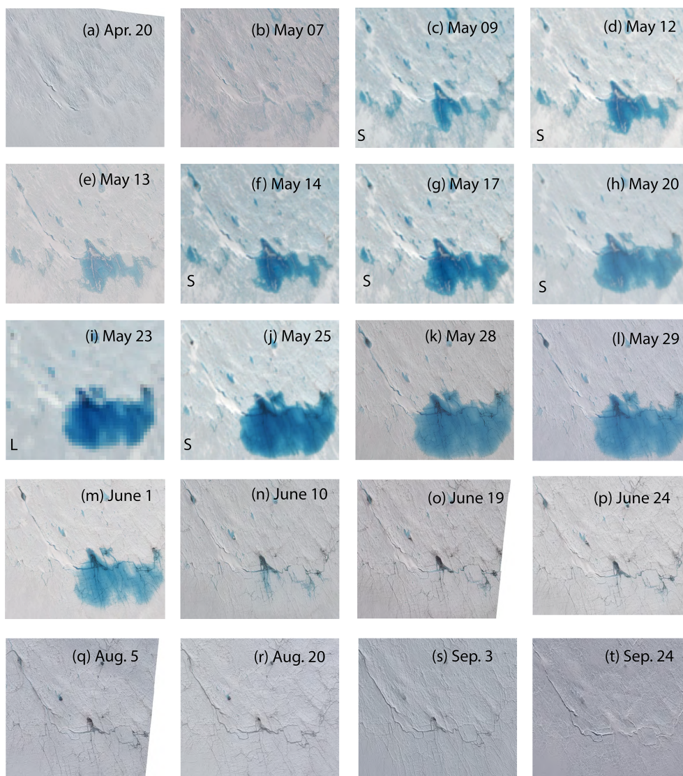
Figure 8. Imagery over Lake Julian shown from 20 April through 24 September 2019. All images use Planet SkySat Visual data unless otherwise indicated by letter on bottom left, with S indicating Sentinel and L indicating Landsat.
