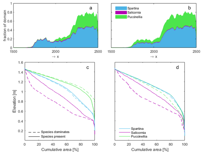
Figure 8. Distribution of three species across domain in S2-scenarios Multi1 (a) and Multi2 (b). Accompanied by hypsometric curves for the three species based on the elevations of cells where the species occurs: Multi1 (c) and Multi2 (d). Solid lines are based on all cells where a species is present; dashed curves are based on only cells where the species dominates (species with the highest fraction prevails). Note: In (d), the solid blue line ( Spartina ) overlaps with the solid green line ( Puccinellia ). X = 1,500 indicates the seaward boundary.
