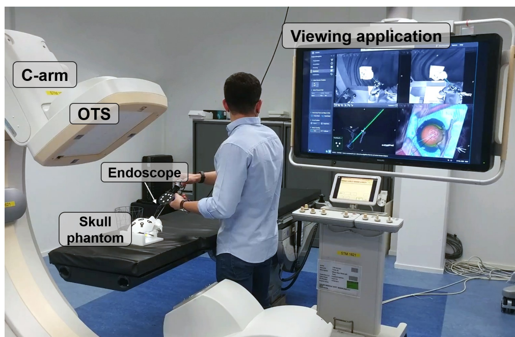
Fig 2. Experimental setup for the study on the skull phantom.
