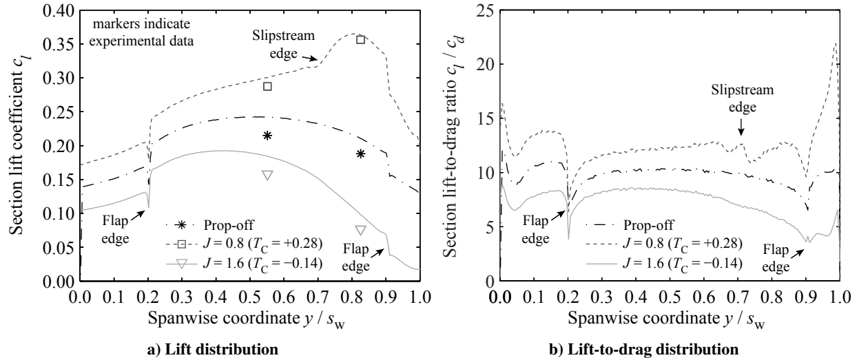
Fig. 13 Effect of propeller thrust setting (inboard-up rotation) on the wing loading distribution at \alpha = 0^\circ (CFD and experimental data).
