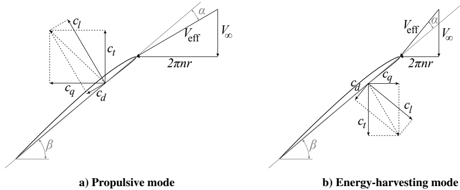
Fig. 1 Velocity triangles at a fixed-pitch propeller blade section in propulsive and energy-harvesting modes.
