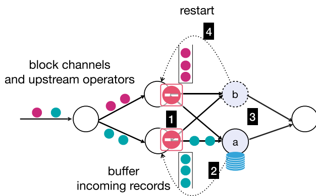
Fig. 8 An example of the partial-pause-and-restart protocol. To move state from operator a to b , the mechanism executes the following steps: (1) Pause a 's upstream operators, (2) extract state from a , (3) load state into b , and (4) send a restart signal from b to upstream operators
