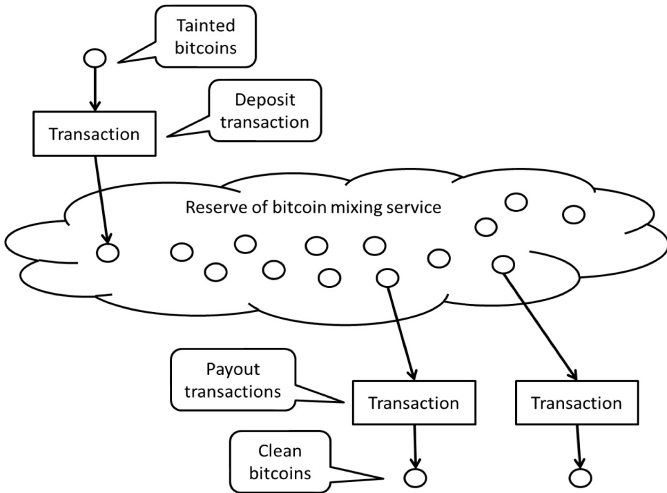
Figure 4.3: A bitcoin mixing service where 'tainted' bitcoins are deposited in the reserve of the mixer, and subsequently 'clean' bitcoins are paid out to the customer
