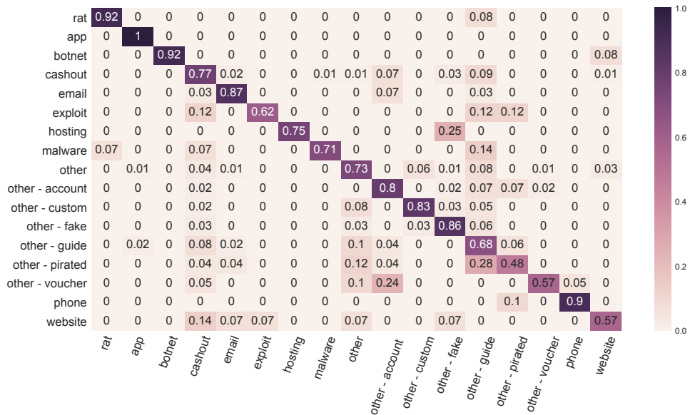
Figure 3.3: Classifier normalized confusion matrix
