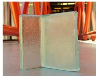
Fig. 1 Welded T-section (left) and fused T-section (right).
