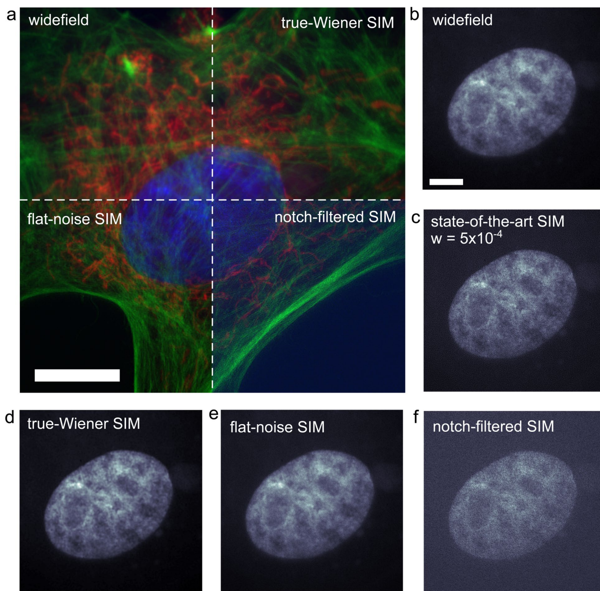
Extended Data Fig. 2 | Multi-color noise-controlled 2D-SIM reconstructions. a , Combined widefield, true-Wiener SIM, flat-noise SIM, and notch-filtered SIM reconstructions of a fluorescent test slide of a bovine pulmonary artery endothelial cell (red channel: mitochondria labeled with MitoTracker Red, green channel: actin labeled with Alexa Fluor 488, blue channel: DNA labeled with DAPI). Note that due to embedding in hardening mounting medium, cells are flattened and 3D nuclear morphology is compromised. b-f , Insets of the DAPI channel comparing state-of-the-art SIM with clear noise amplification artifact to the noise-controlled SIM reconstructions. The SSNR in the DAPI channel is low in this example case, due to reduced signal intensity and compromised morphology. The low SSNR is properly taken into account by the noise-controlled SIM reconstructions, without introducing artifacts, but not by the state-of-the-art SIM reconstruction. Scale bar ( a ) 10 \mu\text{m} , scale bar ( b-f ) 5 \mu\text{m} .
