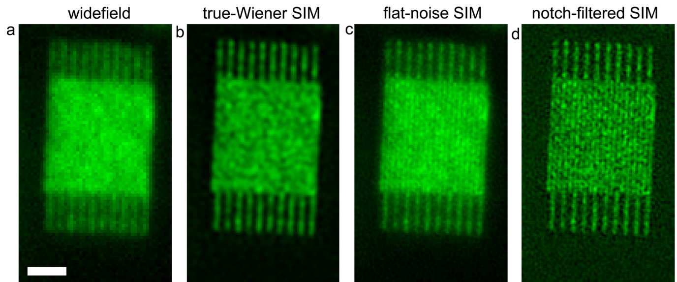
Extended Data Fig. 4 | Flat-noise SIM provides better visibility of high spatial frequency structures. a–d , Widefield, true-Wiener, flat-noise, and notch-filtered SIM reconstructions of a nanofabricated test structure of lines with 140 nm pitch. The line pattern is just visible in flat-noise, and notch-filtered SIM but overshadowed by the noise pattern with uneven distribution of noise over spatial frequencies in true-Wiener SIM. Scale bar 1 \mu\text{m} .
