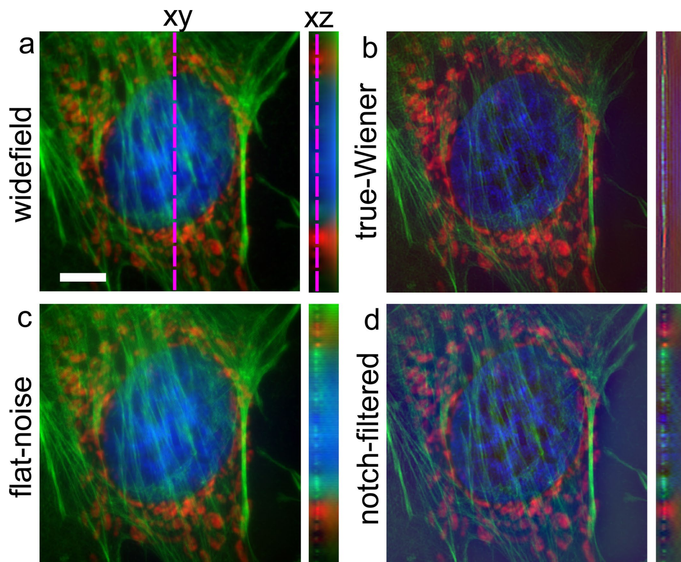
Extended Data Fig. 8 | Widefield and 3D noise-controlled SIM reconstructions of a bovine pulmonary artery endothelial cell. a , Widefield, (b) true-Wiener SIM, (c) flat-noise SIM, (d) notch-filtered SIM (BPAEC, red channel: mitochondria labeled with Alexa Fluor 594, green channel: actin labeled with FITC, blue channel: DNA labeled with DAPI). Scale bar 5 \mu\text{m} .
