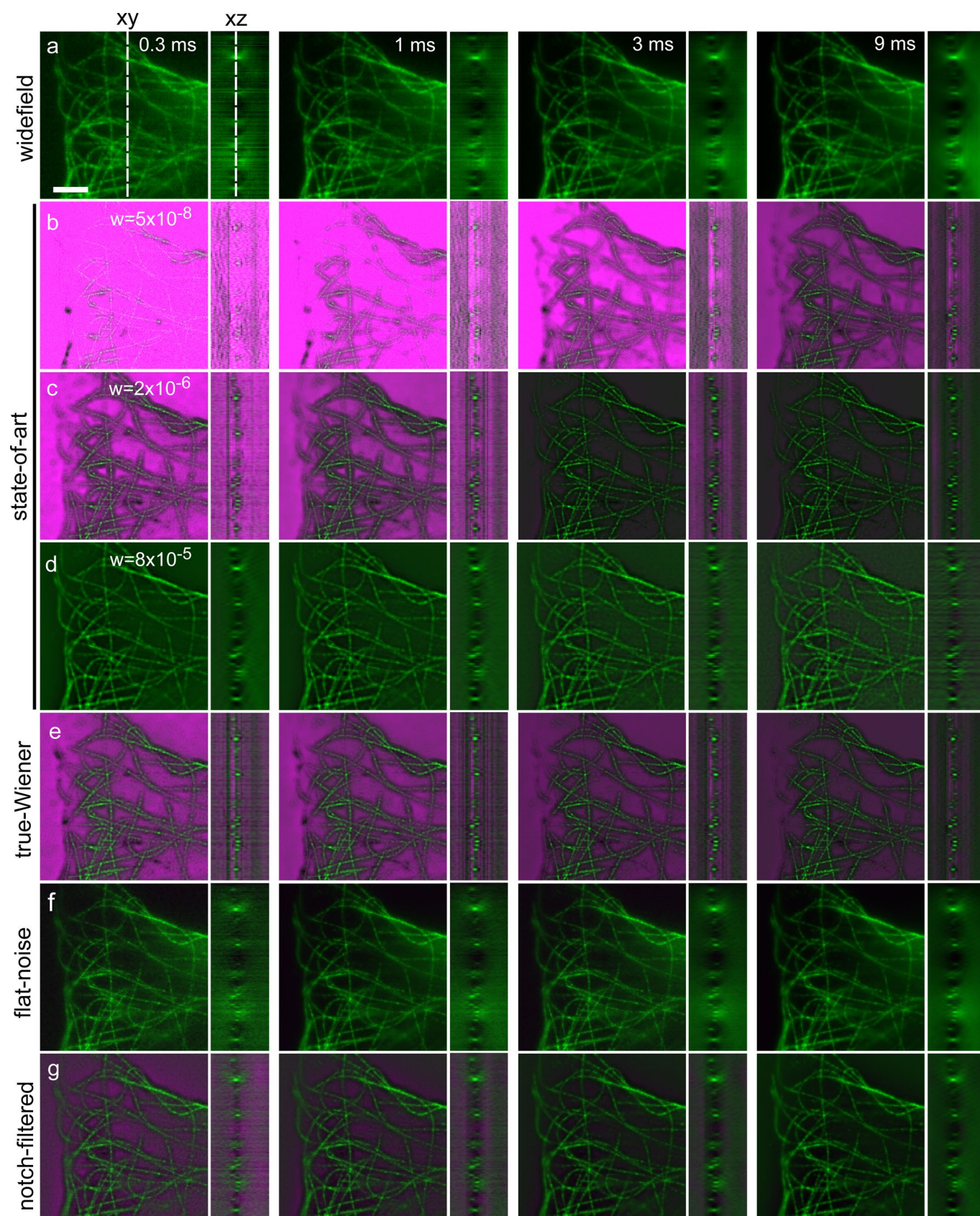
Extended Data Fig. 6 | Cross-sections in xy and yz-planes of 3D-reconstructions of tubulin (green) and noise fraction maps (magenta) for different camera exposure times. a, Widefield, (b–d) state-of-the-art SIM for low, medium and high regularization, (e) true-Wiener SIM, (f) flat-noise SIM, and (g) notch-filtered SIM. The dashed lines in (a) indicate the location of the xz and xy slices. Scale bar 3 \mu\text{m} .
