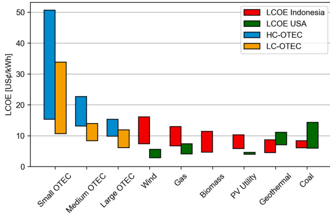
Fig. 5. OTEC's competitiveness against other energy technologies in Indonesia in 2019. Small OTEC < 20 MW, medium OTEC 20 \text{ MW} < P_{net} < 75 MW, large OTEC 75 \text{ MW} < P_{net} < 100 MW. Gas includes open-cycle, closed-cycle, and combined-cycle. Coal refers to subcritical plants. LCOE of competing technologies based on [48] in Indonesia and based on [49] in USA.
