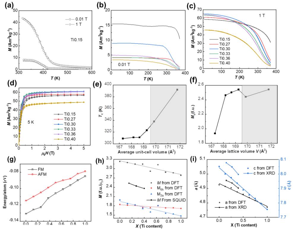
Fig. 6.3. (a) M - T curves for the Ti0.15 sample. (b) M - T curves of Fe_2Hf_{1-x}Ti_x for heating in a magnetic field of 0.01 T and (c) M - T curves of Fe_2Hf_{1-x}Ti_x for heating in a magnetic field of 1 T. (d) M - H curves for Fe_2Hf_{1-x}Ti_x at a temperature of 5 K. (e) T_C as a function of the average unit-cell volume of Fe_2Hf_{1-x}Ti_x . (f) M_s as a function of average unit-cell volume of Fe_2Hf_{1-x}Ti_x . DFT calculation results for the Fe_2Hf_{1-x}Ti_x alloys with: (g) formation energy for the ferromagnetic (FM) and antiferromagnetic (AFM) phase, (h) calculated magnetic moment, and (i) calculated lattice parameters a and c as a function of the Ti content. For the single-phase samples (arc-melted Ti0.15, Ti0.27 and melt-spun Ti0.40), the experimental magnetic moment and lattice parameters are also given for comparison in (h) and (i), respectively.
