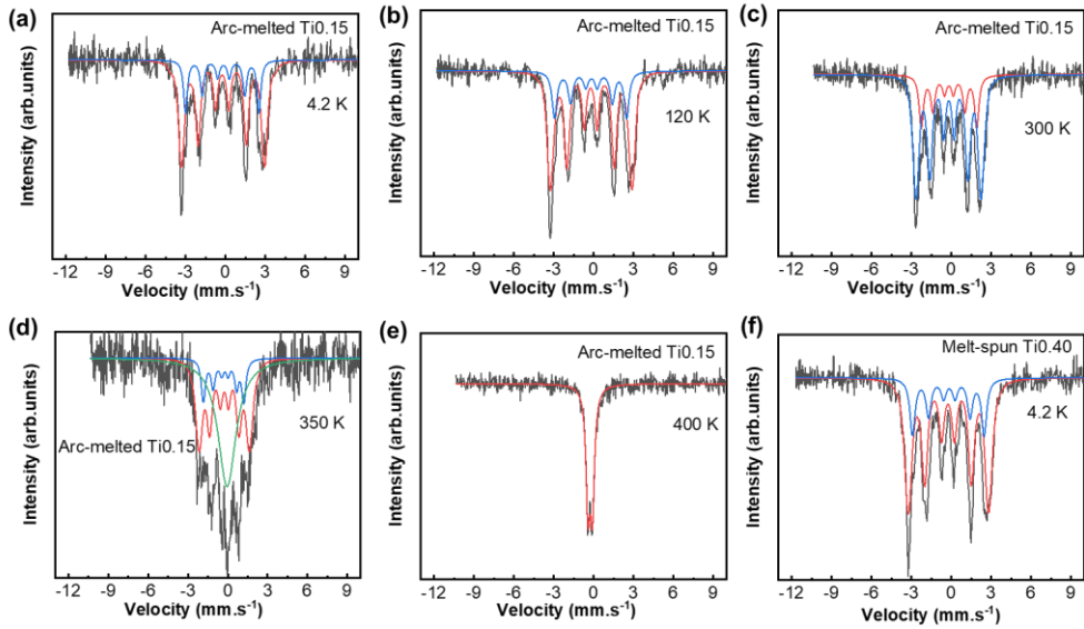
Fig. 6.7. Mössbauer spectra of the arc-melted Ti 0.15 sample at (a) 4.2 K, (b) 120 K, (c) 300 K, (d) 350 K, (e) 400 K. (f) Mössbauer spectra of the melt-spun Ti 0.40 sample at 4.2 K. The black line represents the experimental spectrum.
