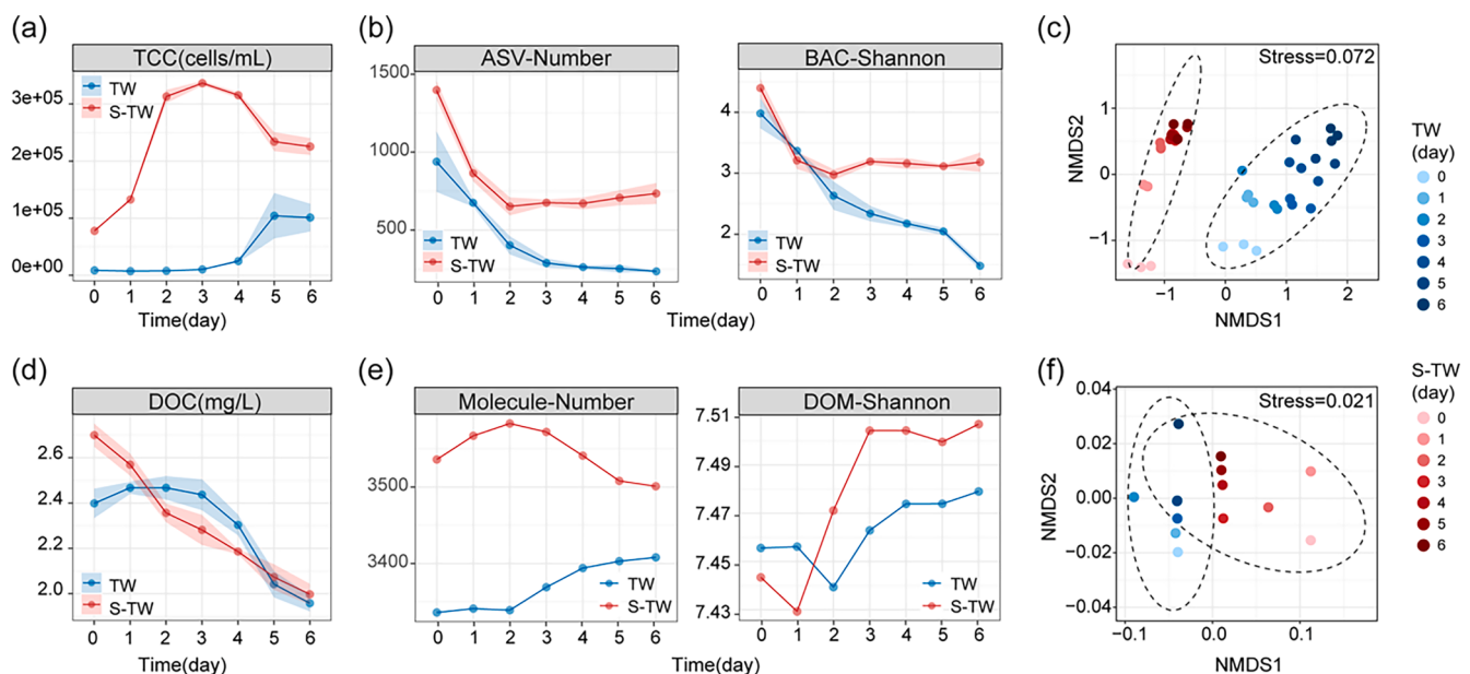
Fig. 1. Seven days' dynamic of bacteria and dissolved organic matter. (a) changes of biomass quantified by total cell count (TCC); (b) alpha diversity of bacterial community; (c) NMDS plots based on Bray-Curtis dissimilarity of bacterial community; (d) changes of dissolved organic carbon concentrations (DOC); (e) alpha diversity of DOM; (f) NMDS plots based on Bray-Curtis dissimilarity of DOM. Lines with ribbons in subfigures (a, b, d) indicate means \pm standard deviation (SD) ( n = 3 ).
