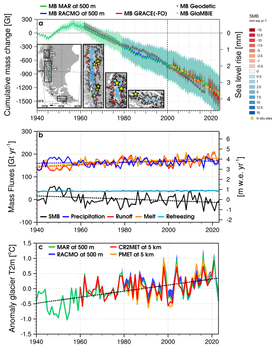
Fig. 1 | Long-term mass loss of Patagonian glaciers. a Monthly cumulative mass change ( MB = SMB - D ) of Patagonian glaciers. Mass change is estimated as the difference between downscaled surface mass balance (SMB) from MAR (green line, 1940–2023) and RACMO (blue line, 1979–2023) at 500 m resolution, and solid ice discharge estimates ( D ) from 1968–1999 9 and 2000–2019 12 , assuming that these remain valid pre-1968 (1940–1999) and post-2019 (2000–2023), respectively. The vertical dashed line marks the transition between these two solid ice discharge products. Geodetic mass change from Zemp et al. (2019) 9 (1961–2016), GRACE/GRACE-FO satellite mass change (2002–2023), and from the latest GlaMBIE assessment (2000–2023) 8 are shown in grey, red and orange respectively. Coloured bands represent uncertainties. Inset maps show averaged MAR SMB at 500 m (1940–2023) with a zoom in on three major Patagonian icefields: Northern
