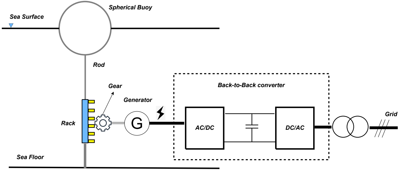
Fig. 1: Schematic of the spherical heaving point absorber with a bottom-founded geared rotary PM generator [10].
