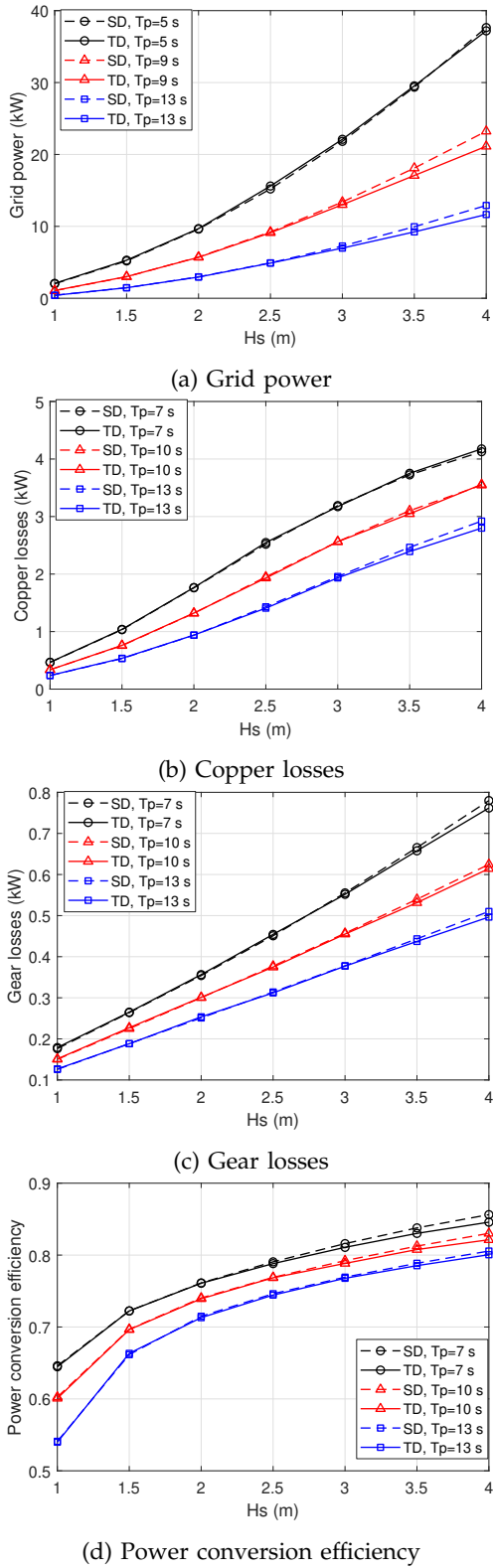
Fig. 4: Grid power, copper losses and power conversion efficiency of the WEC in different wave states and the relative errors of the SD model to the TD model. ( B_{pto} = 60 kNs/m)
