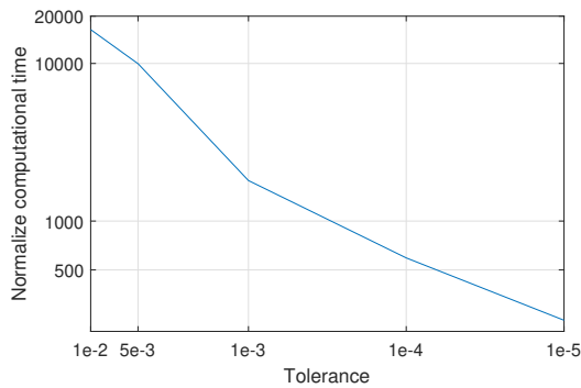
Fig. 6: The computational time of the SD W2W model to that of the TD W2W model. The simulation case was run with inputs of H_s = 3m and T_p = 7s .
