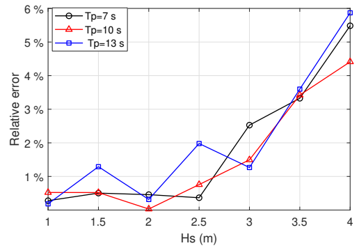
Fig. 5: The relative errors of the established SD W2W model to the TD W2W model with regard to the grid power estimation.
