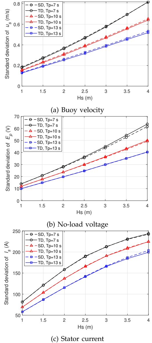
Fig. 3: The standard deviation of the responses of the WEC in different wave states of the SD W2W model to the TD W2W model. ( B_{pto} = 100 kNs/m)
