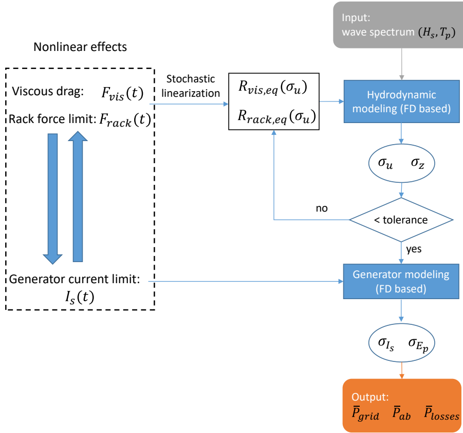
Fig. 2: Diagram of the proposed SD wave-to-wire modeling.
