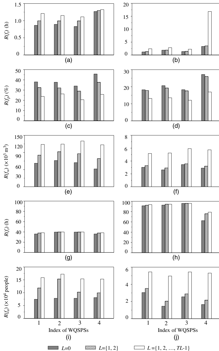
Fig. 5. Robustness values of the four WQSPSs for the two case studies: (a) JYN; (b) ZHN; (c) JYN; (d) ZHN; (e) JYN; (f) ZHN; (g) JYN; (h) ZHN; (i) JYN; and (j) ZHN.
