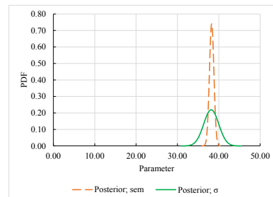
Figure 10: The posterior PDF based on the standard deviation of the mean (Posterior; sem) and the overall standard deviation of the population (Posterior; \sigma ).
