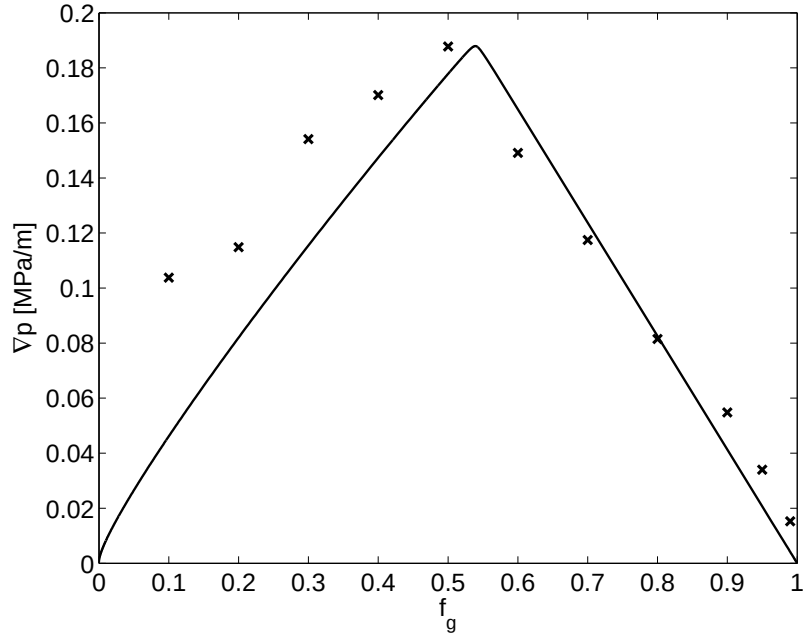
Figure 3.5: Model fit to data of Ma et al. (2013) using only the water-saturation-dependent function (F2). Data points are shown as crosses. The solid line shows the model fit.
