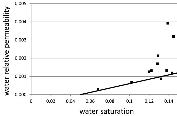
Figure 4.8: Data for k_{rw}(S_w) computed from \nabla p and S_w data of Ma et al. (2013). A linear function works reasonably well for the four lowest- f_w data most important to gas injection in SAG (see Table B.3 in Appendix B).
