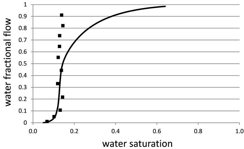
Figure 4.13: STARS model fit to data of Ma et al. (2013) over entire range of f_w adjusted to fit mobility data in middle range of data: f_{mmob} = 40,000 , f_{mdry} = 0.13 , epdry = 150 .
