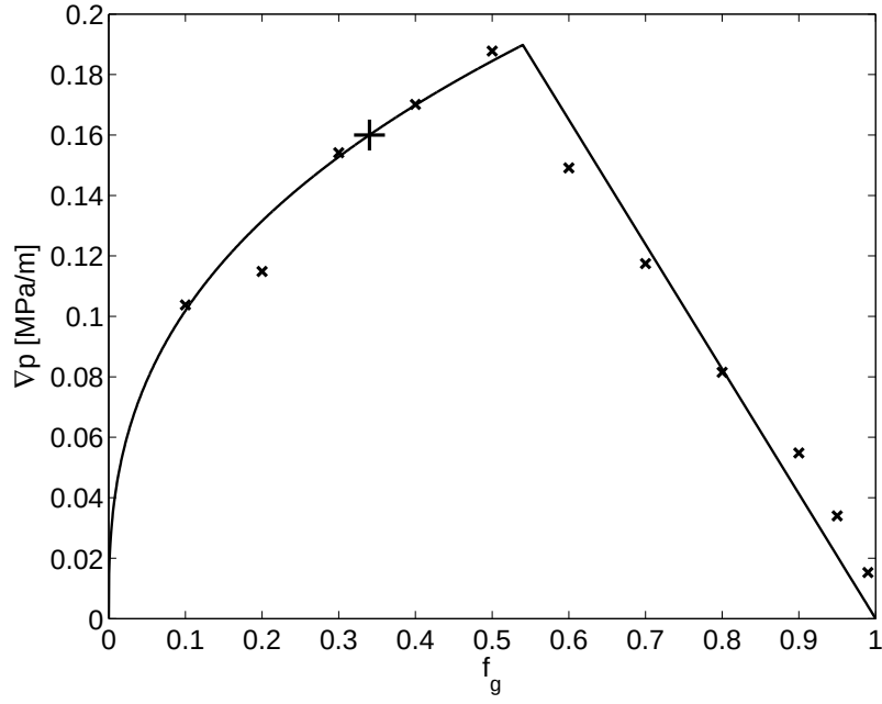
Figure 3.6: Model fit to data of Ma et al. (2013) including the capillary-number-dependent function ( F_5 ) in the low-quality regime. Data points in the low- and high-quality regimes are shown by crosses. The solid line shows the model fit. The '+' sign is the chosen value of (f_g^+, \nabla p(f_g^+)) .
