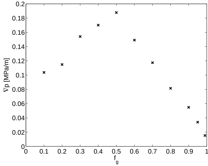
Figure 3.3: Scan of foam data at fixed total superficial velocity, after Ma et al. (2013)
