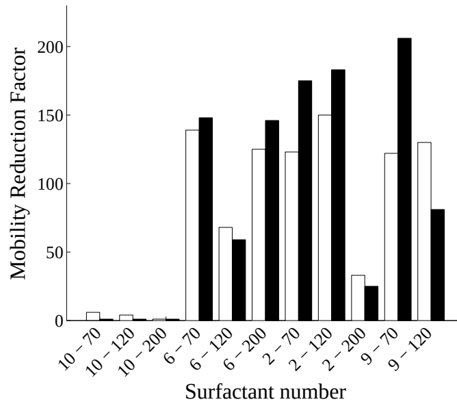
Figure 2.7: Measured mobility reduction factors ( MRF ) in the lipophilic bead pack without (white bars) and with oil (black bars). MRF values are shown here on a linear scale to emphasize the difference between measurements with and without oil. On the horizontal axis, the first label is the surfactant number and the second the brine salinity [ \times 1000 ppm].
