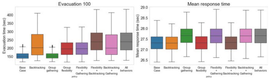
Fig. 6 Results for the multi variant behavior testing. The evacuation times (left) and response time (right) for each combination
