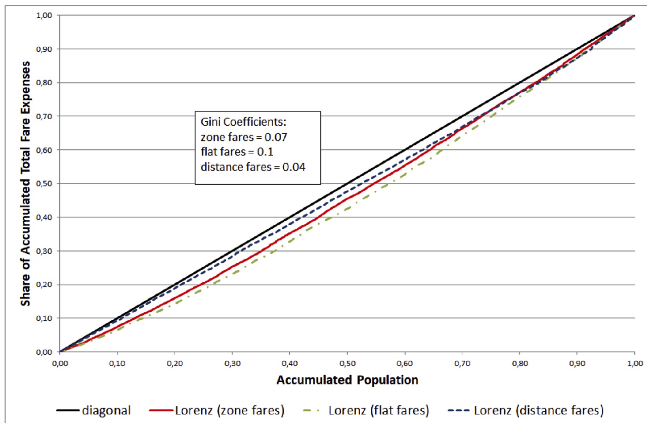
Fig. 7. The Lorenz curves and their corresponding Gini-coefficients for the total amount of fares paid for public transport rides.
