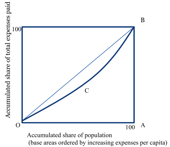
Fig. 2. Schematic illustration of the Lorenz-curve, the area between the diagonal and the Lorenz-curve (C) as a share of the area under the diagonal is the Gini-coefficient.
