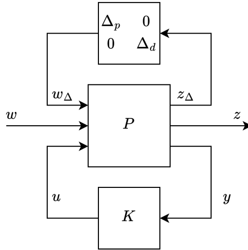
Figure 3 General LFT with controller and structured uncertainty
