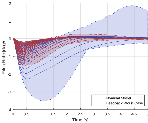
Figure 16 Linear response of a step input disturbance of 0.2 [deg] with all flight points and bounds of a Monte Carlo simulation of 100 random sampled models per flight point
