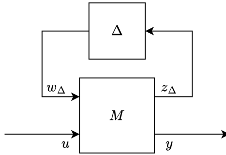
Figure 7 Upper LFT of a plant with structured uncertainty
