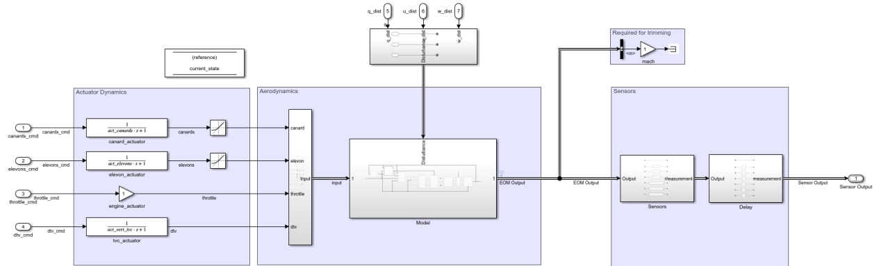
Figure 5 Longitudinal open-loop ADMIRE Aircraft in Simulink
