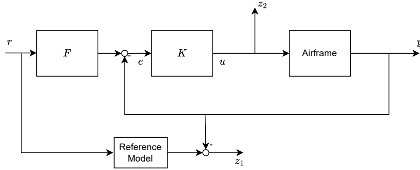
Figure 11 Block diagram of the feed-forward synthesis
