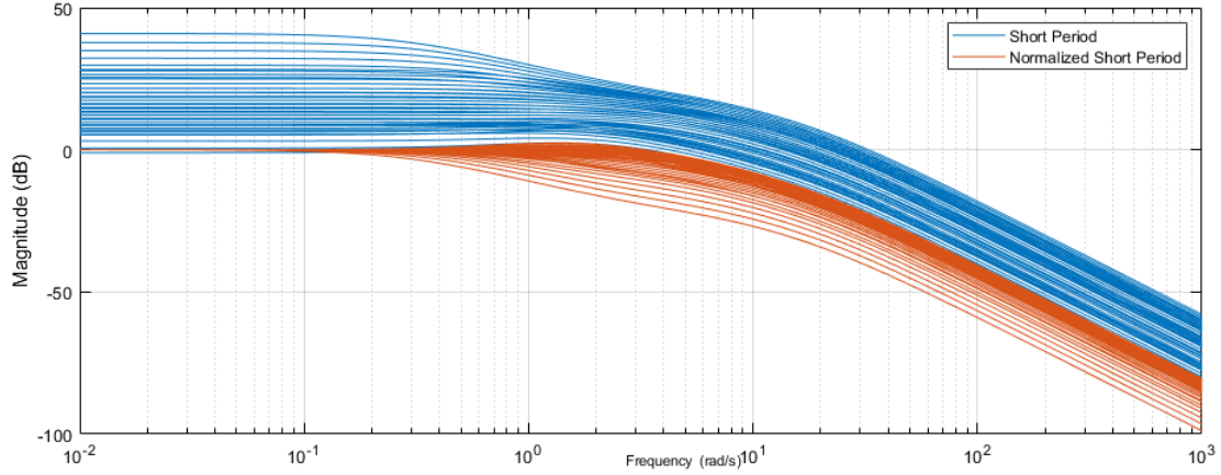
Figure 9 Bode plot of the magnitude of a normalized short period model and regular
