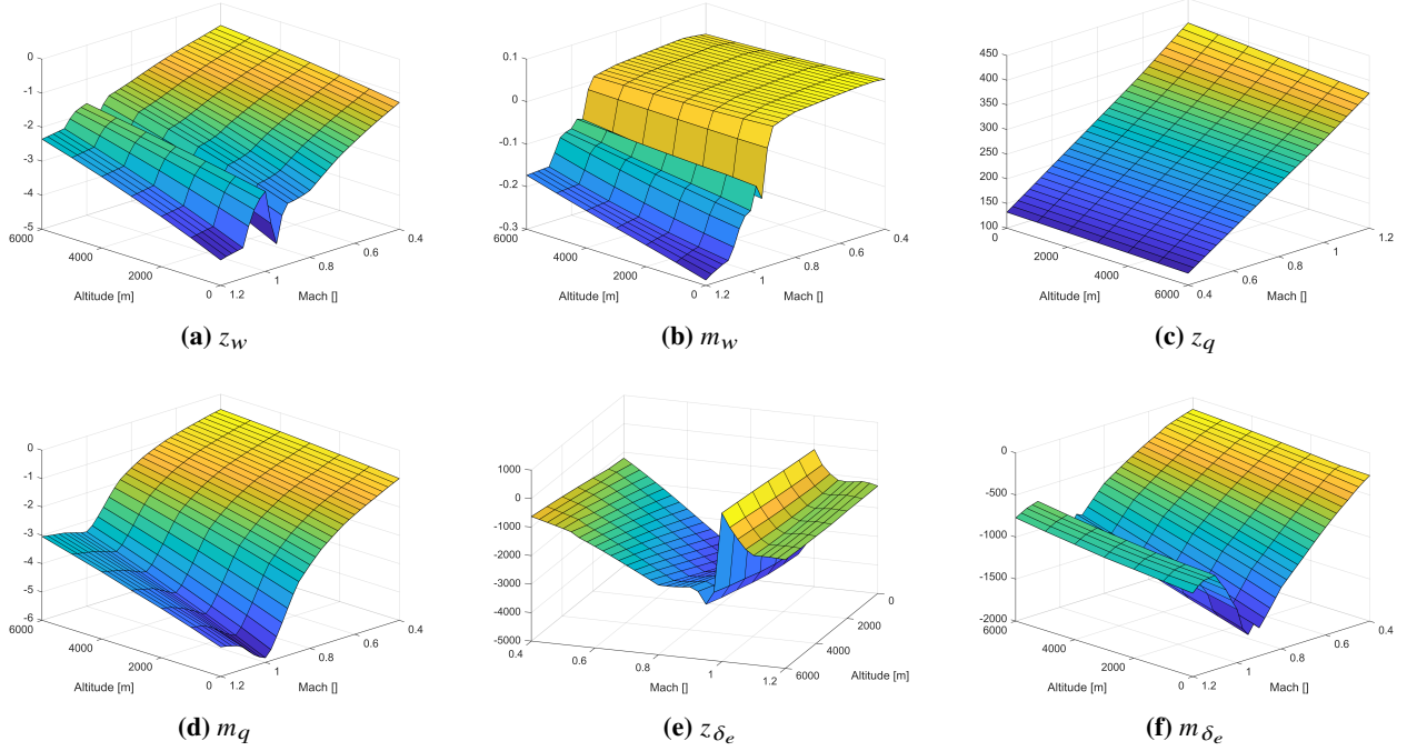
Figure 6 Short Period reduction parameters for the ADMIRE
