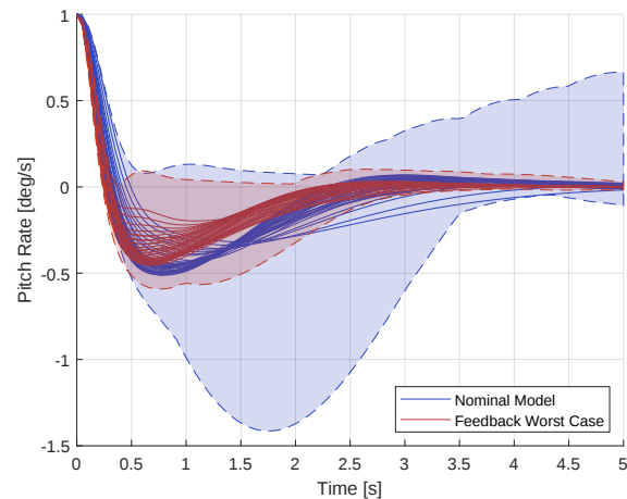
Figure 17 Linear response of a step output disturbance of 1 [deg/s] with all flight points and bounds of a Monte Carlo simulation of 100 random sampled models per flight point
