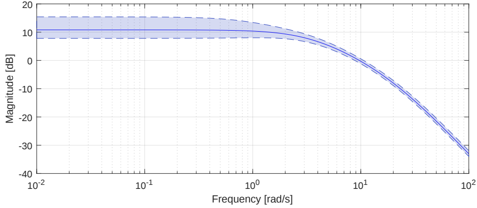
Figure 8 Example of the short period bode plot with its nominal model and a uncertainty component generated by sampling the upper LFT with 100 samples
