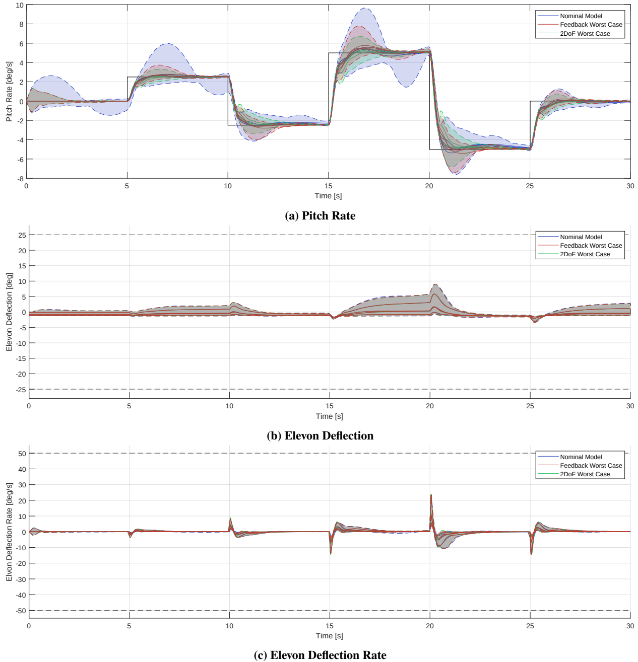
Figure 18 Non-Linear Simulation of the synthesised controller, with all flight points and bounds of a Monte Carlo Simulation of 100 random sampled models per flight point (shaded)
