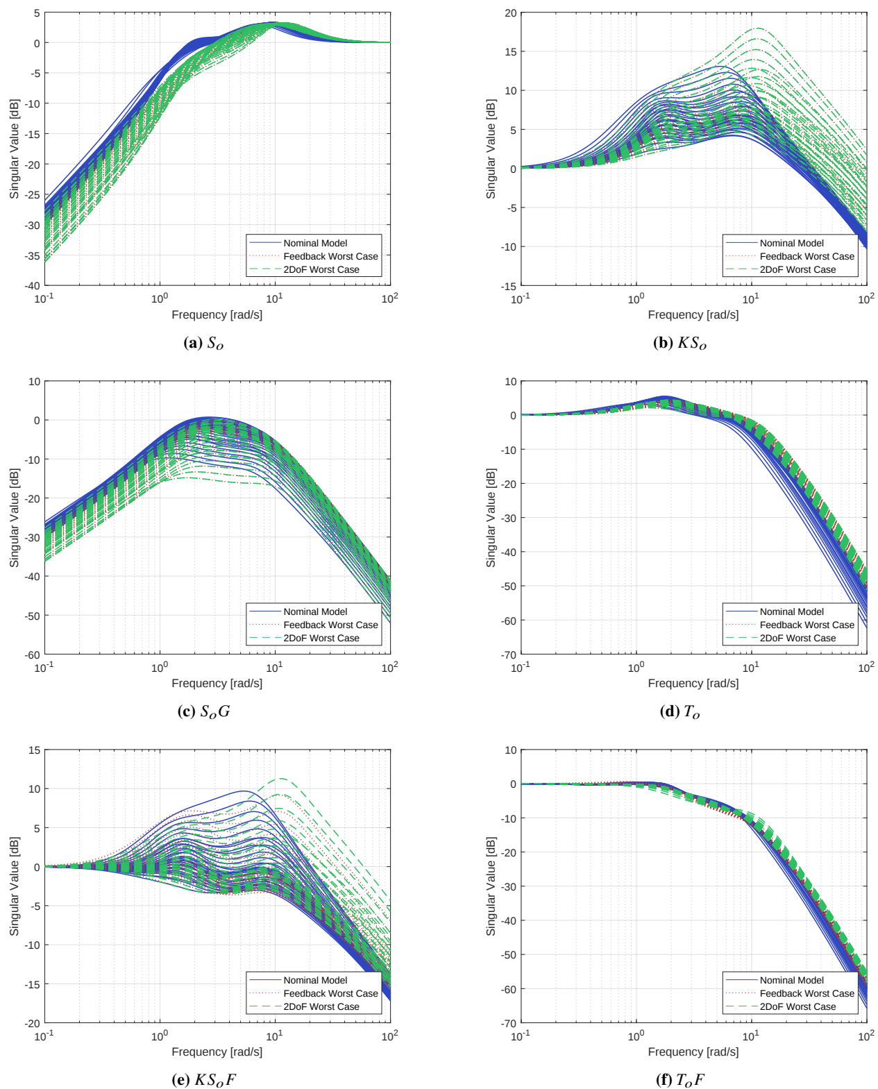
Figure 13 Gang of six of all gain scheduled flight points with nominal plant conditions
