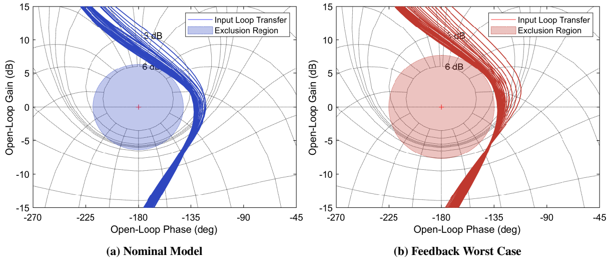
Figure 14 Nichols plots of all flight points. Exclusion Region [shaded] is based on the worst-case disk margin of all flight points
