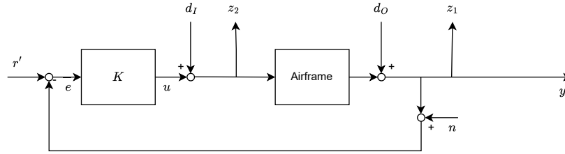
Figure 10 Feedback Synthesis Structure
