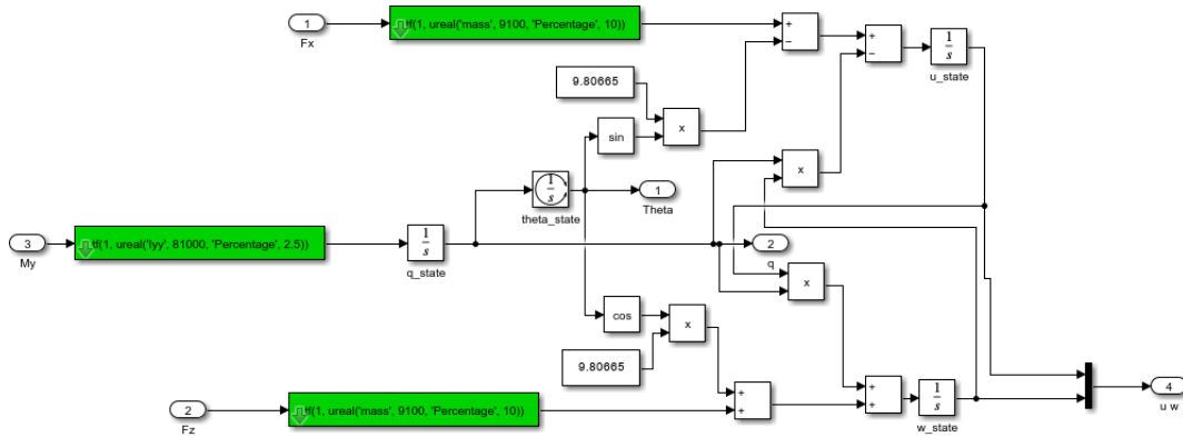
Figure 4 Simulink implementations of the EOM for the longitudinal dynamics
