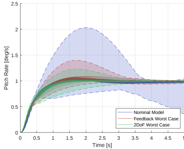
Figure 15 Linear step response of all flight points and bounds of a Monte Carlo simulation of 100 random sampled models per flight point
