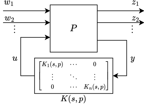
Figure 2 Standard closed-loop LFT with multi-objective signals and tunable controller
