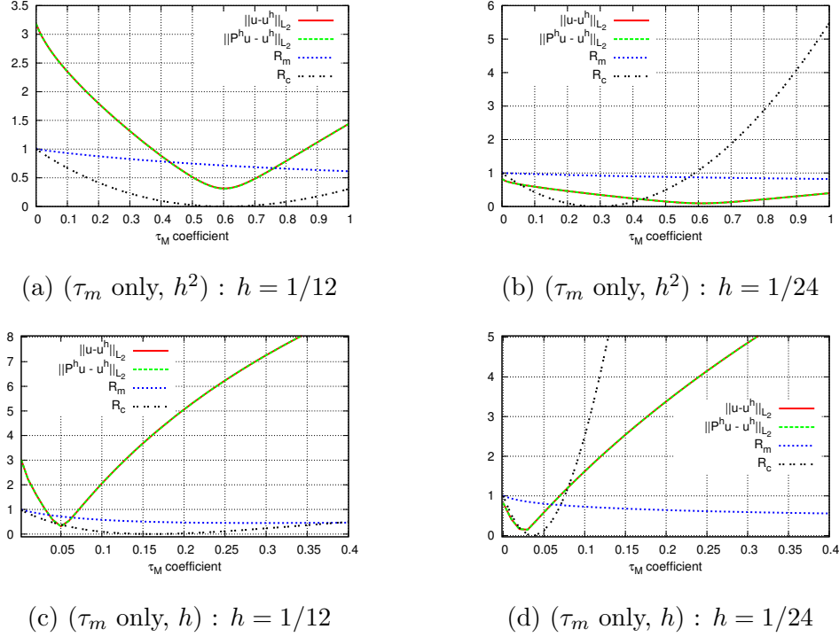
Figure 2: Plot of R_m , R_c , L_2 error and \|\mathbb{P}^h u - u^h\| for different value of c_1 for the (\tau_m \text{ only}, h^2) and (\tau_m \text{ only}, h) models with h = 1/12 and h = 1/24 .
