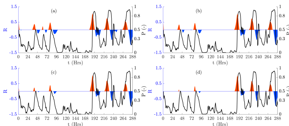
Figure 3. Detected normalized power ramps for the period of 20 to 31 May 2015 for a_{max} = 20 with discrimination levels, W_T^* of: (a) 10% (b) 5% (c) 2% and (d) 1%. Ramp-up events are shown in red and ramp-down events in blue.
