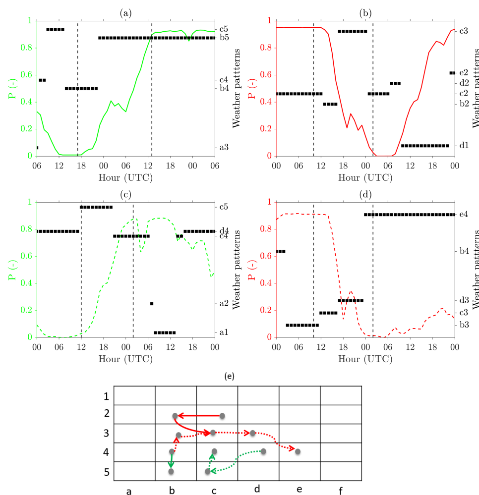
Figure 8. Weak wind power ramp cases and associated weather patterns: (a) R1 (b) R2 (c) R3 (d) R4, and (e) a sketch of the weather-pattern transitions for R1 (solid green line), R2 (solid red line), R3 (green dashed line) and R4 (red dashed line). R1–R4 periods are shown in Table 1. The vertical black dash lines in the (a–d) indicate the detected start and end time of the ramps.
